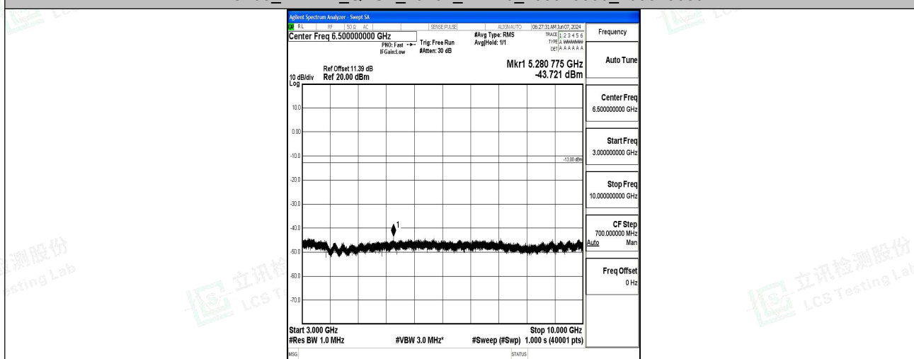
Band5_1.4MHz_QPSK_20407_1RB#0_3000~10000_3000~10000
