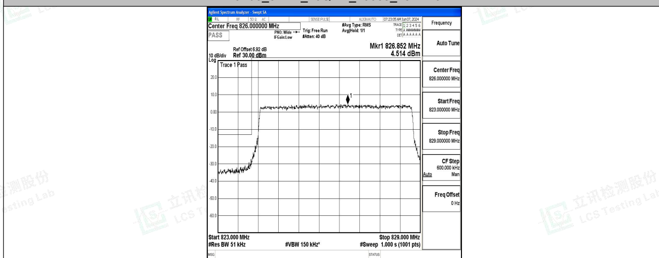
Band5_5MHz_QPSK_20425_25RB#0
