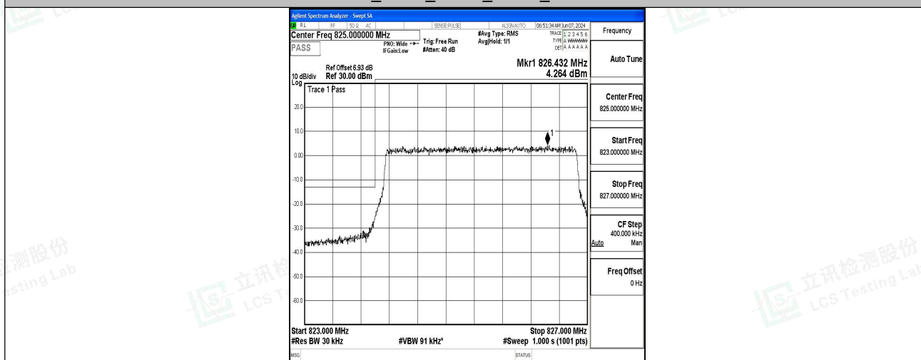
Band5_3MHz_16QAM_20415_15RB#0
