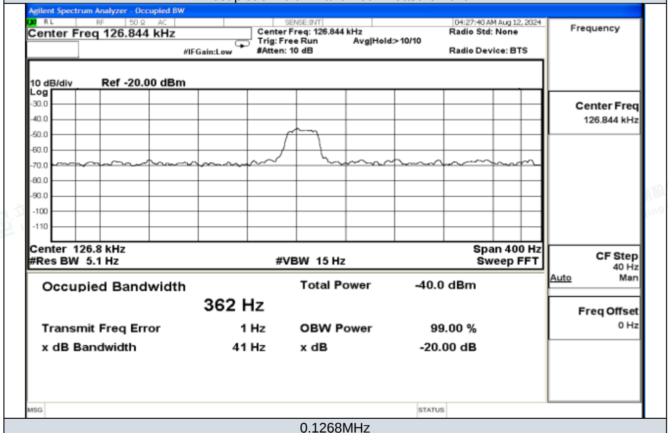
Test plot of 20 dB Bandwidth Measurement
