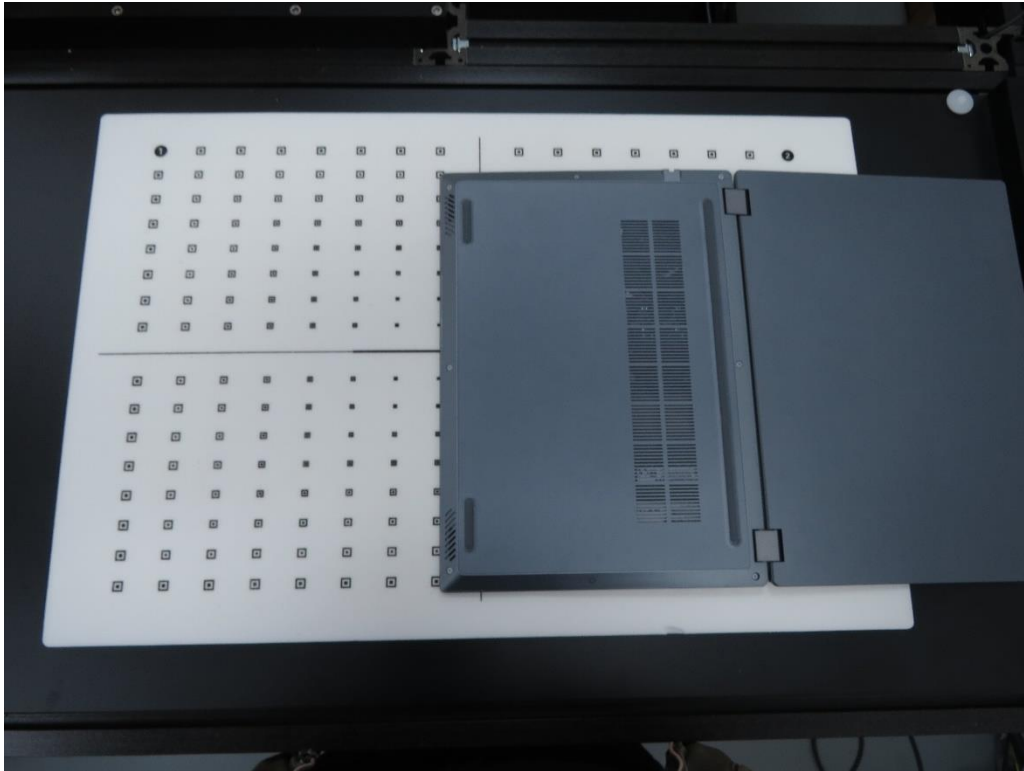
Picture 2: Back Side, the distance from EUT to the Phantom is 2mm
