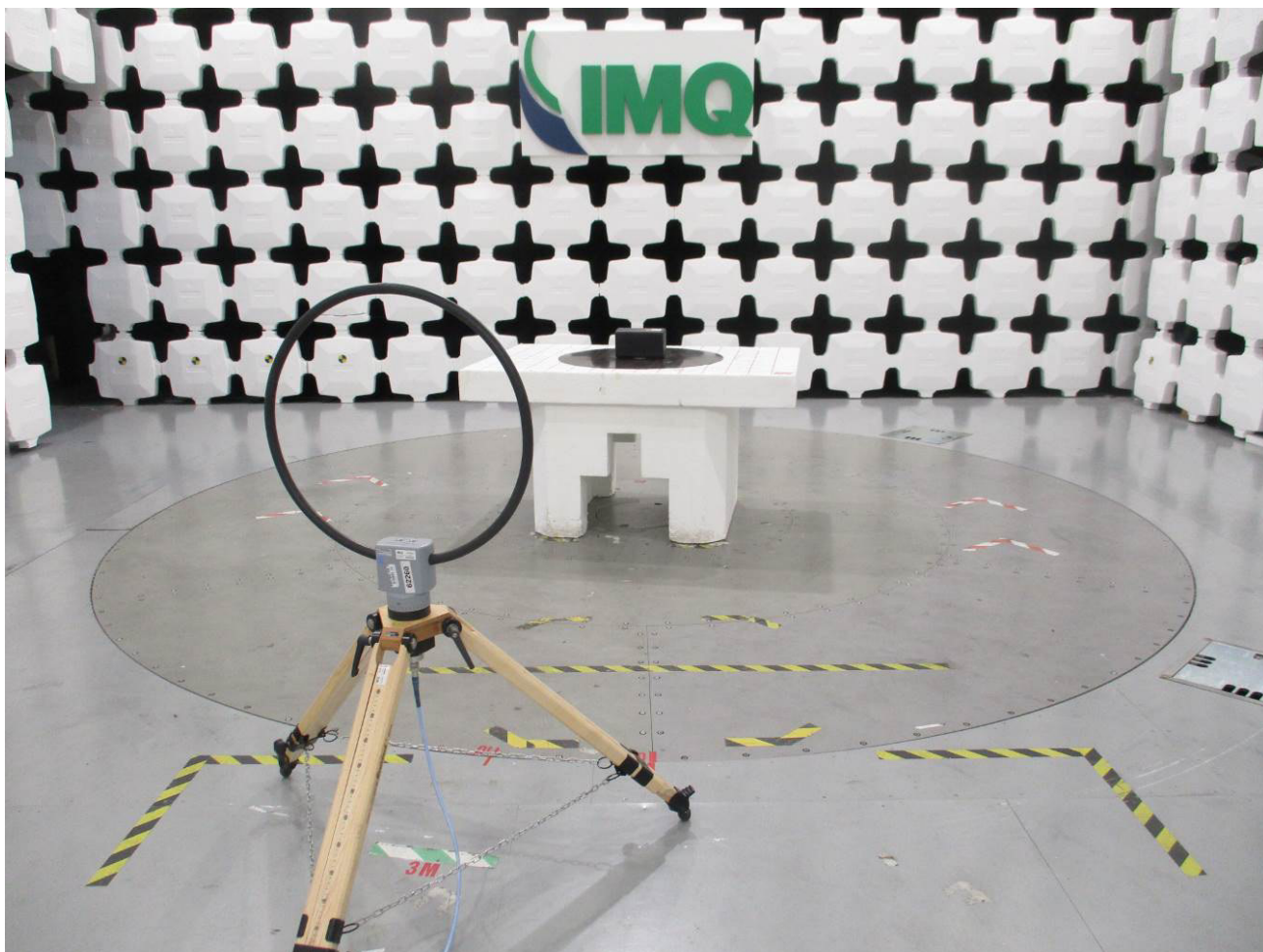
TEST SET-UP – Radiated tests 9kHz-30MHz
