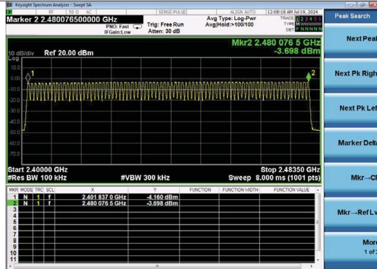
GFSK Modulation
