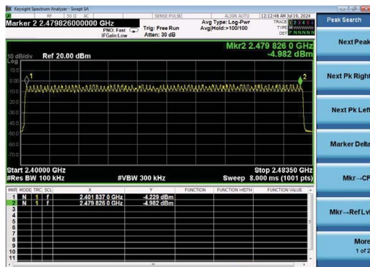
8-DPSK Modulation
