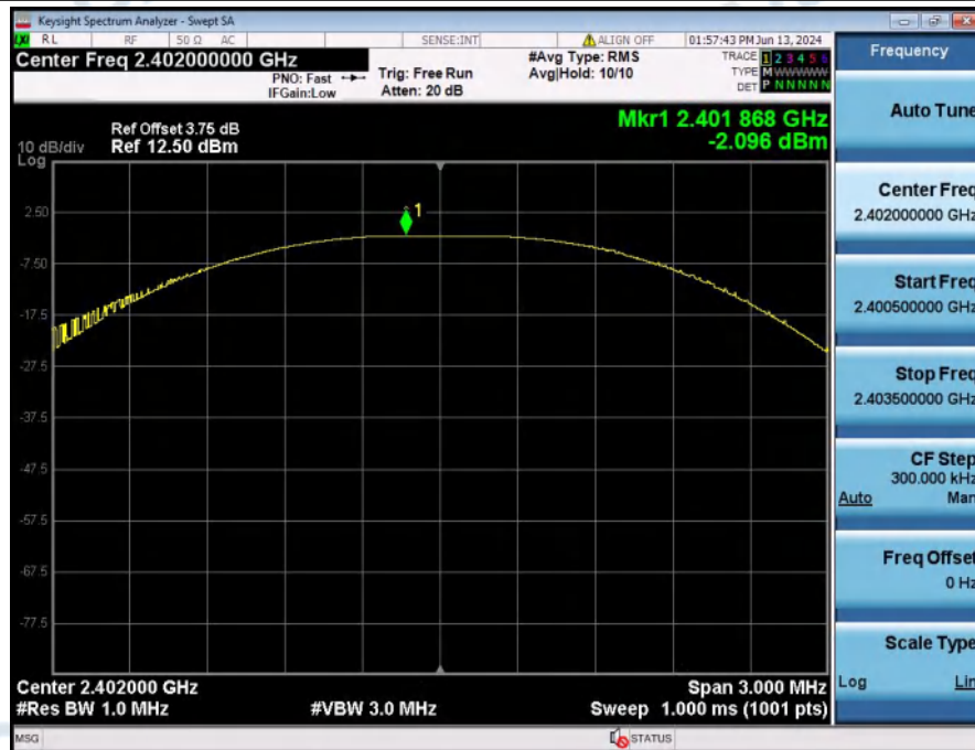
Peak_Output_Power_NVNT_ANT1_1-DH5_2402_00
