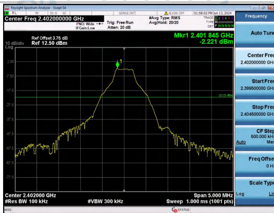
2_Spurious_Emissions_NVNT_ANT1_1-DH5_2402_00
