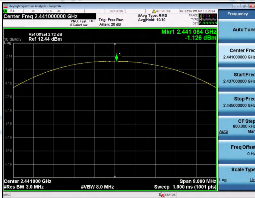
Peak_Output_Power_NVNT_ANT1_2-DH5_2441_00
