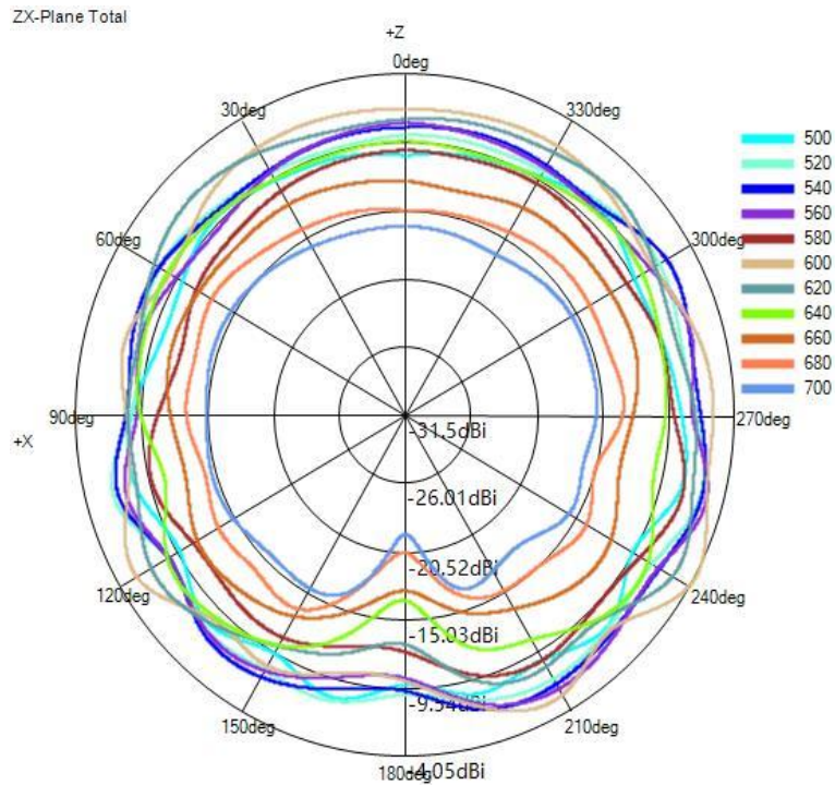
(1) X-Z Plane(unit:dBi):
