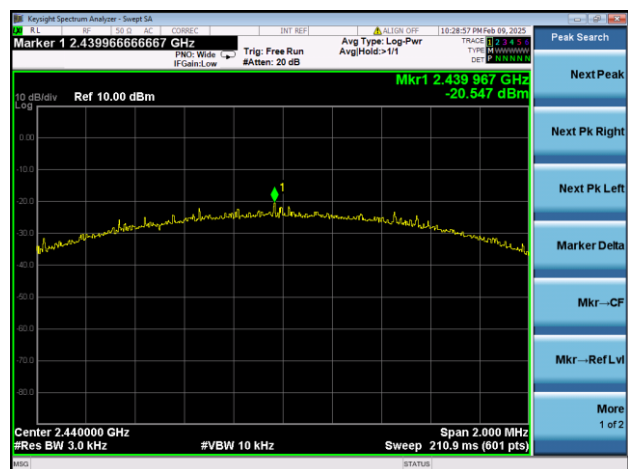
GFSK (BLE 2Mbps) MIDDLE CHANNEL
