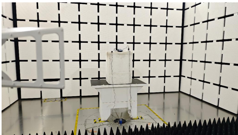
Above 1GHz-RF
