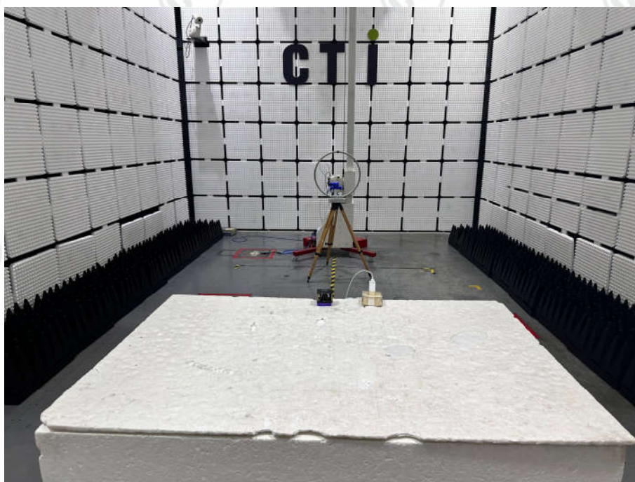
Radiated Emissions Test Setup (9kHz-30MHz)Mode b to Mode d
