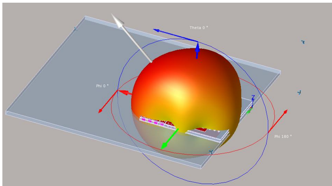
Directivity at Channel 9
