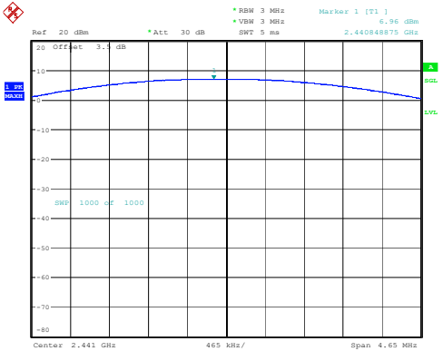
DH1_Middle 6.96dBm
