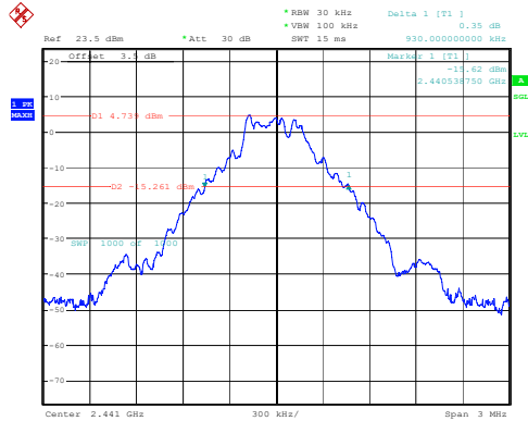
DH1_Middle 0.930MHz
