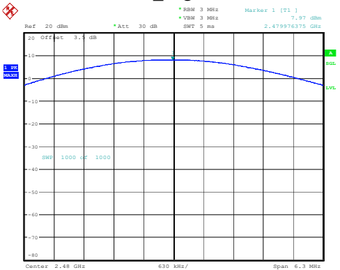
2DH1_High 7.97dBm
