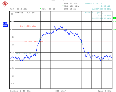
3DH1_High 1.234MHz
