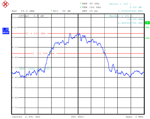
2DH1_Middle 1.256MHz
