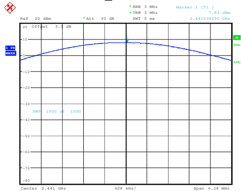
2DH1_Middle 7.83dBm
