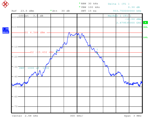
DH1_High 0.934MHz
