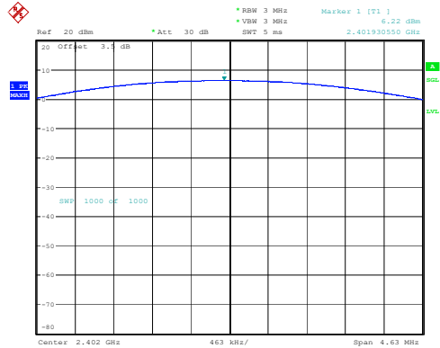
DH1_Low 6.22dBm
