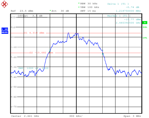
3DH1_Middle 1.219MHz
