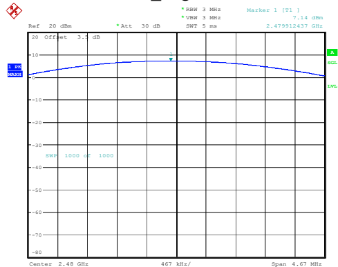
DH1_High 7.14dBm
