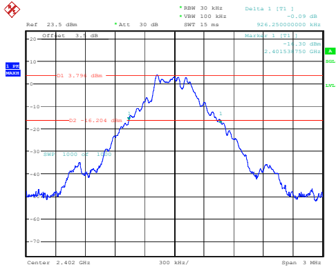
DH1_Low 0.926MHz
