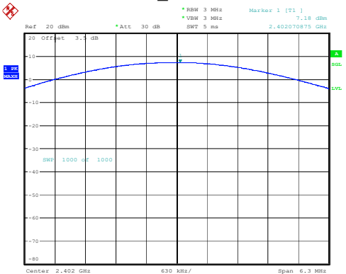
2DH1_Low 7.18dBm
