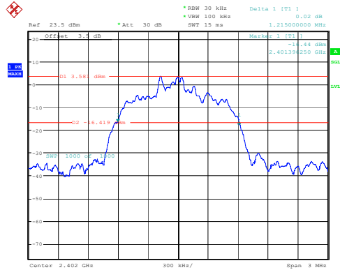
3DH1_Low 1.215MHz
