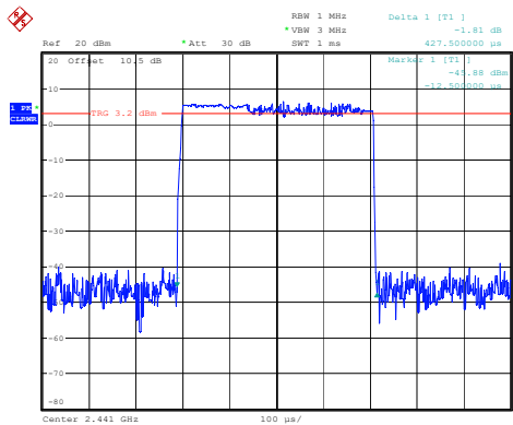
8DPSK_Hopping_3DH1 0.428ms
