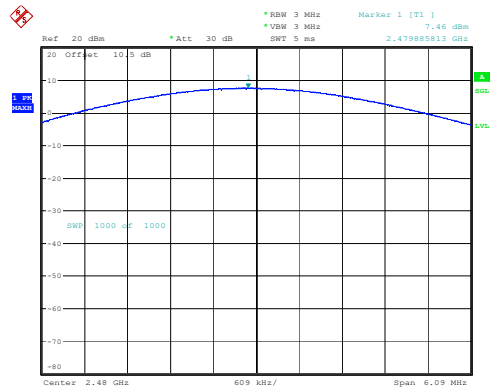
8DPSK_High 7.46dBm
