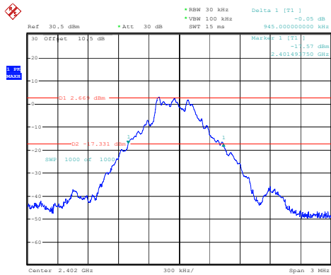
GFSK_Low 0.945MHz
