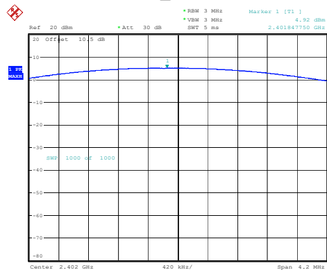
GFSK_Low 4.92dBm
