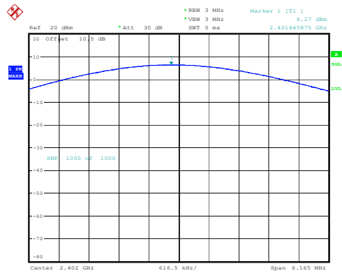
8DPSK_Low 6.27dBm
