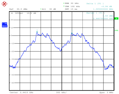
GFSK_Middle 1.005MHz
