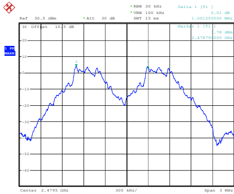
GFSK_High 1.001MHz
