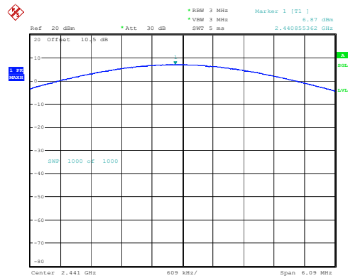
8DPSK_Middle 6.87dBm
