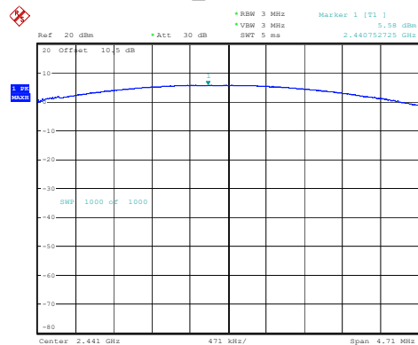
GFSK_Middle 5.58dBm
