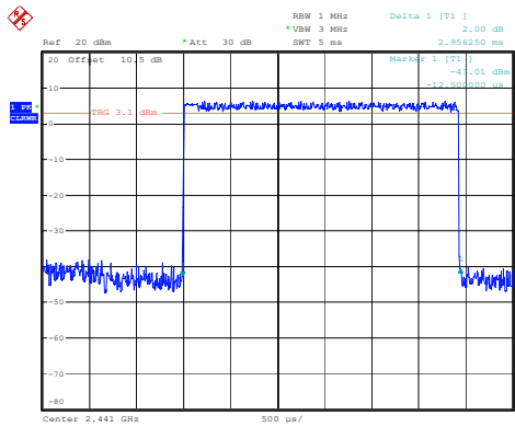
8DPSK_Hopping_3DH5 2.956ms
