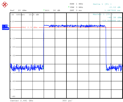
8DPSK_Hopping_3DH3 1.688ms
