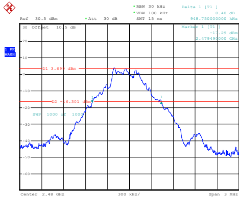
GFSK_High 0.949MHz
