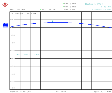
GFSK_High 6.08dBm
