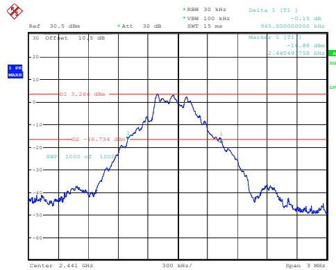
GFSK_Middle 0.945MHz
