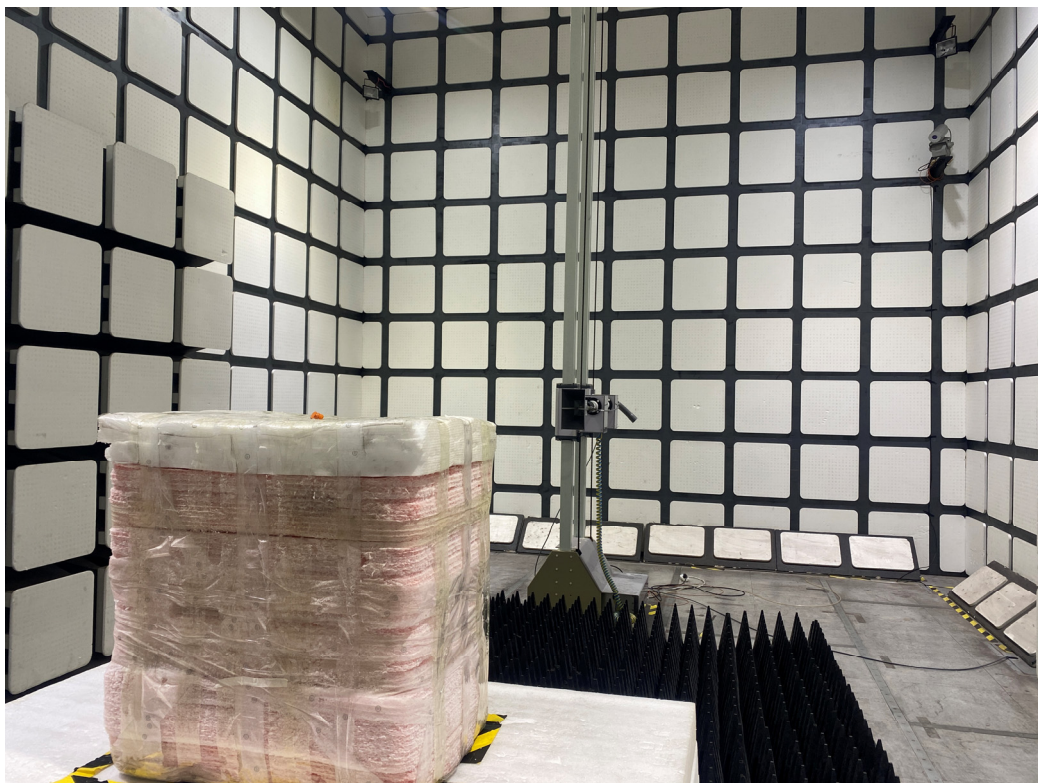
Radiated Emissions View (Above 1 GHz)
