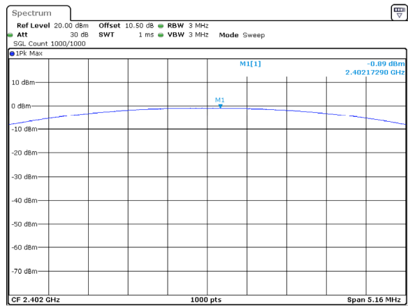
GFSK_Low -0.89dBm
