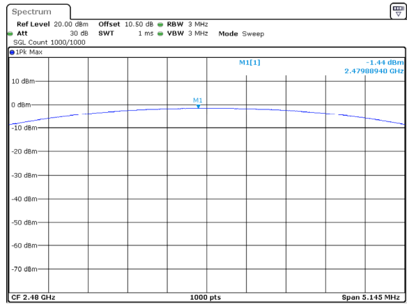
GFSK_High -1.44dBm
