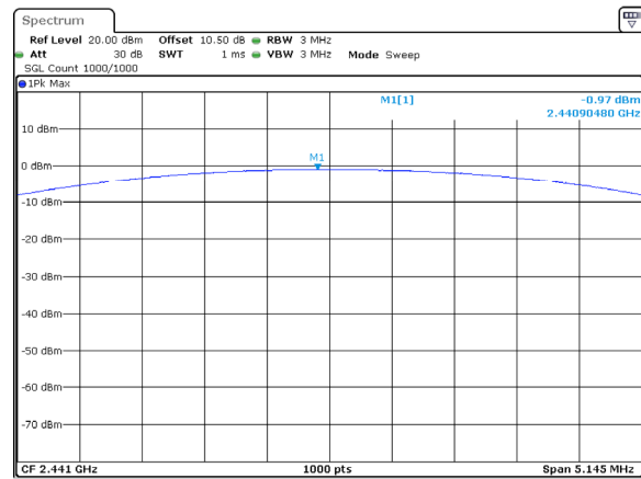
GFSK_Middle -0.97dBm
