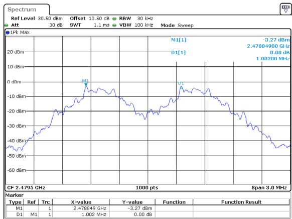
GFSK_High 1.002MHz
