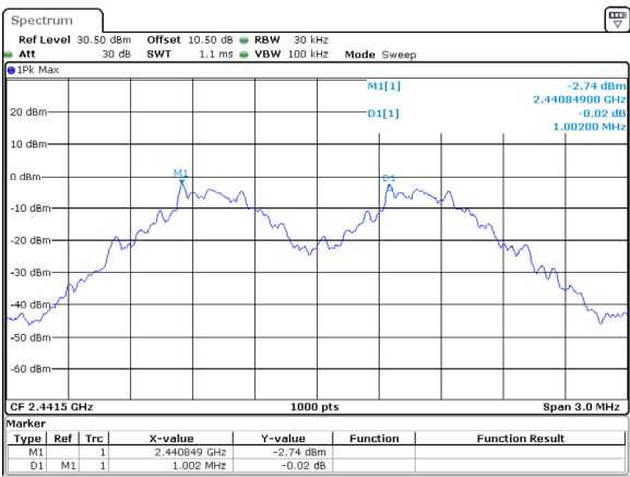
GFSK_Middle 1.002MHz
