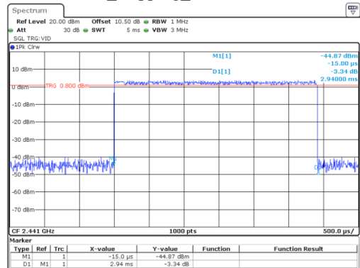
8DPSK_Hopping_3DH5 2.940ms
