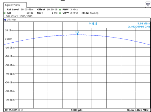
8DPSK_Low 5.01 dBm
