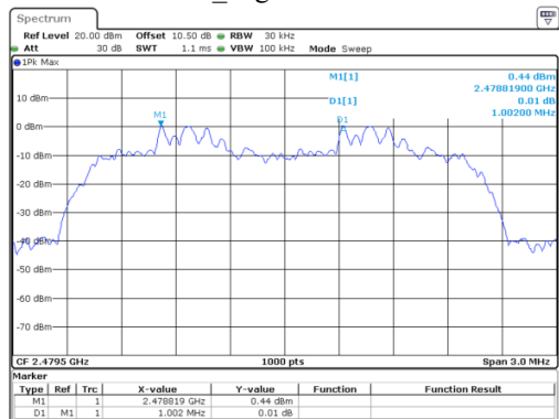
8DPSK_High 1.002 MHz
