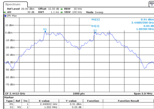
GFSK_Middle 1.002 MHz
