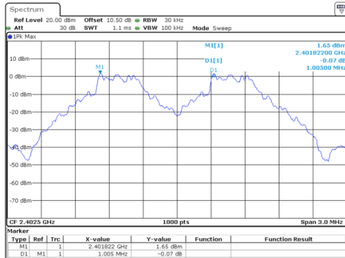
GFSK_Low 1.005 MHz
