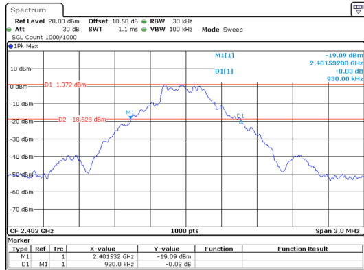
GFSK_Low 0.930 MHz
