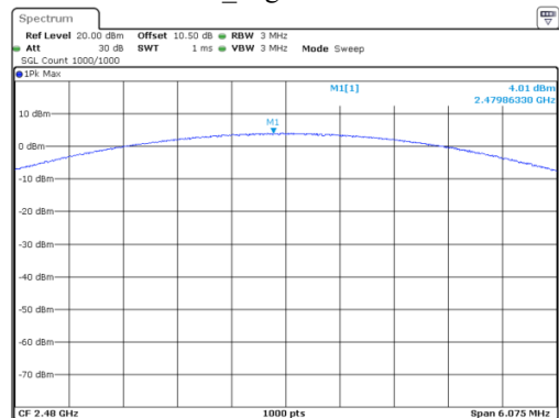
8DPSK_High 4.01 dBm
