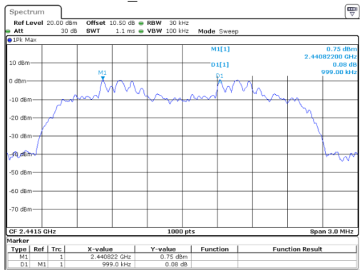
8DPSK_Middle 0.999 MHz
