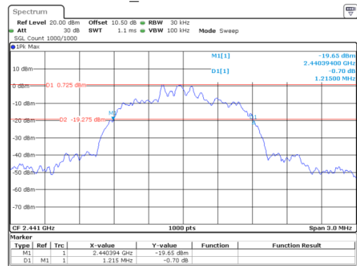
8DPSK_Middle 1.215 MHz
