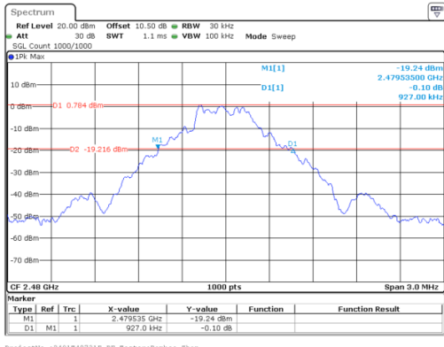
GFSK_High 0.927 MHz
