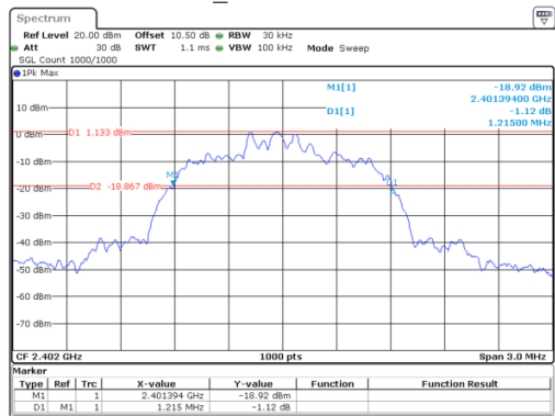
8DPSK_Low 1.215 MHz
