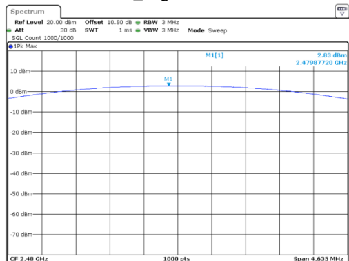
GFSK_High 2.83 dBm
