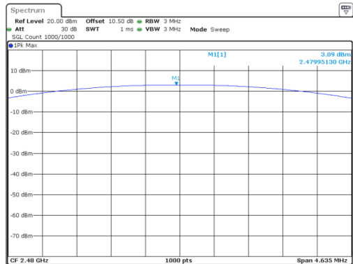
GFSK_High 3.09 dBm
