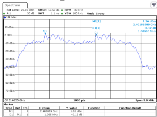
8DPSK_Low 1.005 MHz
