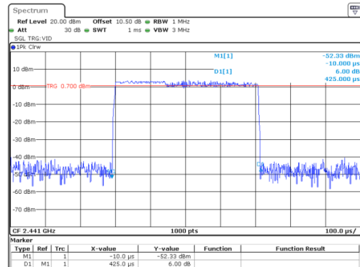
\pi/4 -DQPSK_Hopping_2DH1 0.425ms
