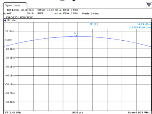
8DPSK_High 4.24 dBm
