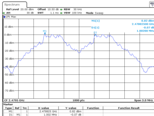
GFSK_High 1.002 MHz
