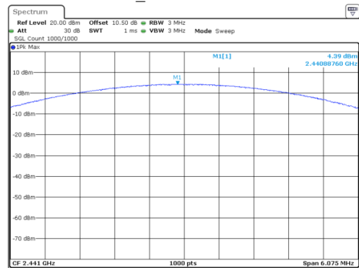
8DPSK_Middle 4.39 dBm
