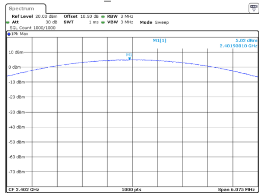
8DPSK_Low 5.02 dBm
