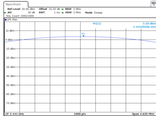
GFSK_Middle 3.50 dBm
