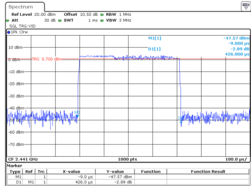
8DPSK_Hopping_3DH1 0.426ms
