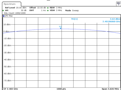
GFSK_Low 3.63 dBm
