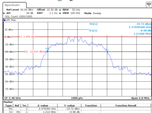
8DPSK_High 1.215 MHz
