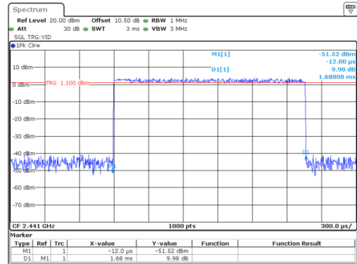
8DPSK_Hopping_3DH3 1.680ms
