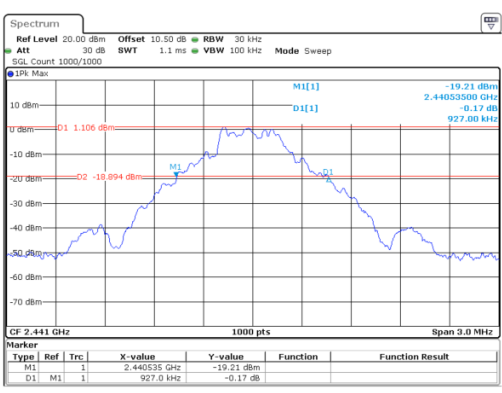
GFSK_Middle 0.927 MHz
