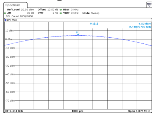
8DPSK_Middle 4.52 dBm
