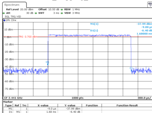
\pi/4 -DQPSK_Hopping_2DH3 1.680ms
