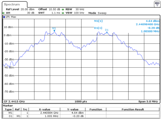
GFSK_Middle 1.005MHz
