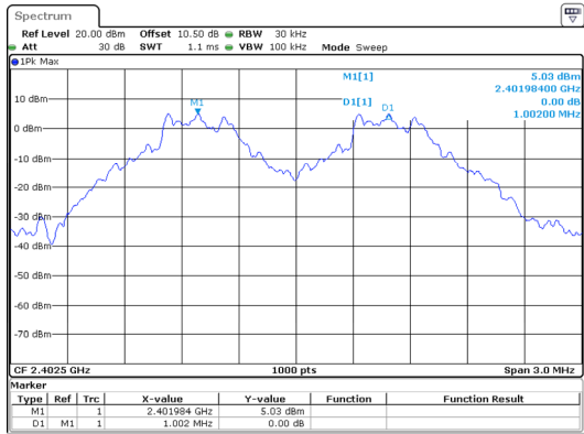
GFSK_Low 1.002MHz
