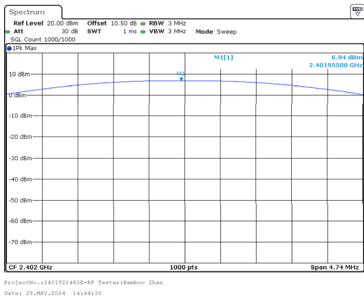
GFSK_Low 6.94dBm
