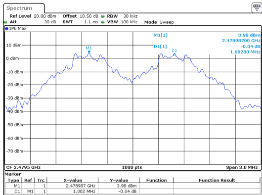
GFSK_High 1.002MHz
