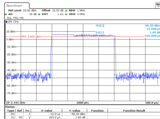
\pi/4 -DQPSK_Hopping_2DH1 0.425ms
