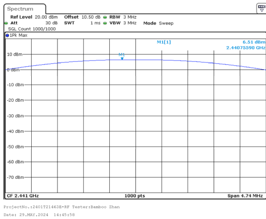
GFSK_Middle 6.51dBm
