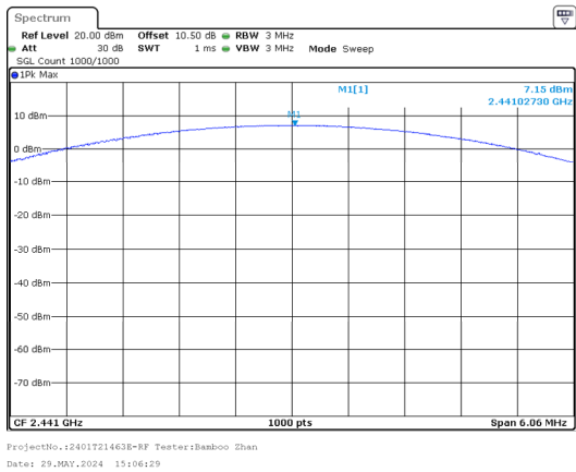
8DPSK_Middle 7.15dBm
