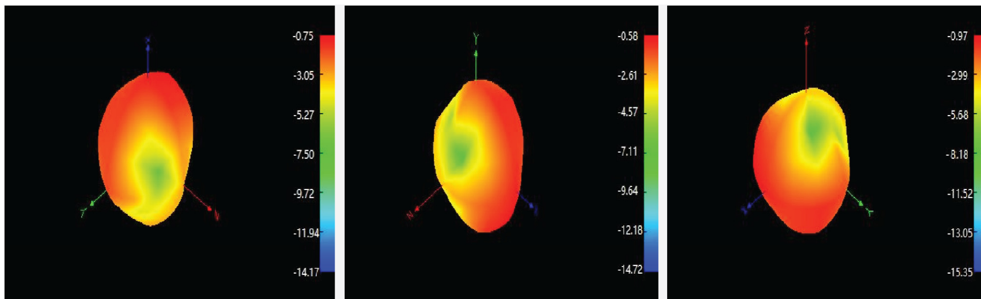
3D Radiation Pattern for 2450MHz
