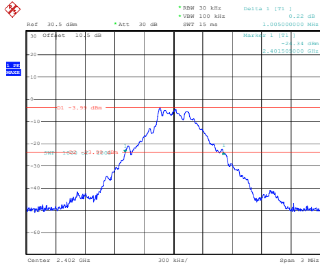
DH1_Low 1.005MHz
