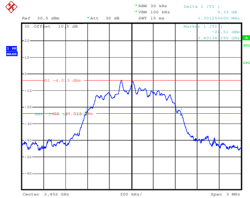
2DH1_Low 1.301MHz
