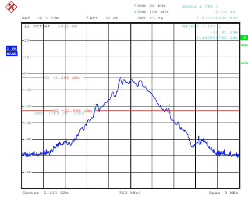
DH1_Middle 1.031MHz
