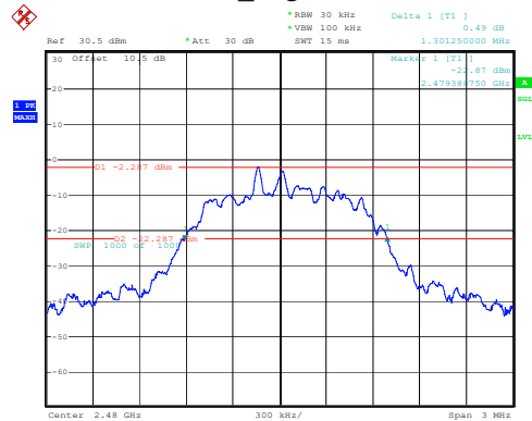
2DH1_High 1.301MHz
