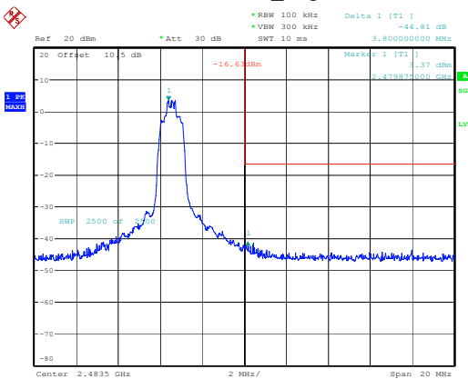
3DH1_High
