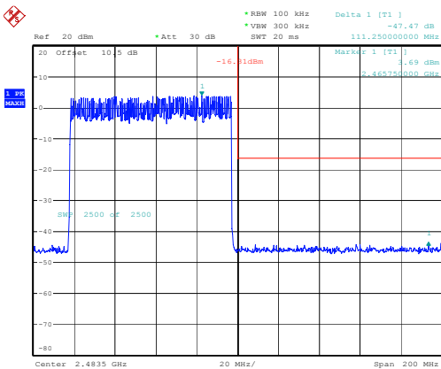
2DH1_Hopping_Upper
