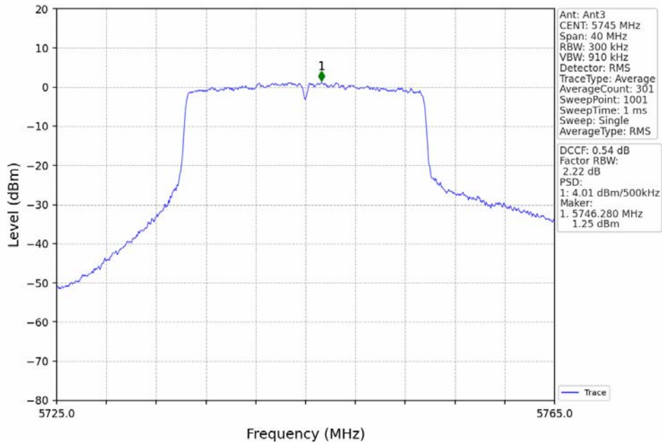
802.11ax(HEW20)_LCH_5745MHz_RU242_Left_MIMO_NTNV
