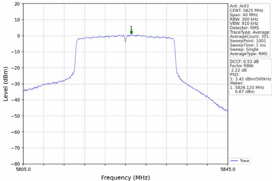
802.11ax(HEW20)_HCH_5825MHz_RU242_Left_MIMO_NTNV
