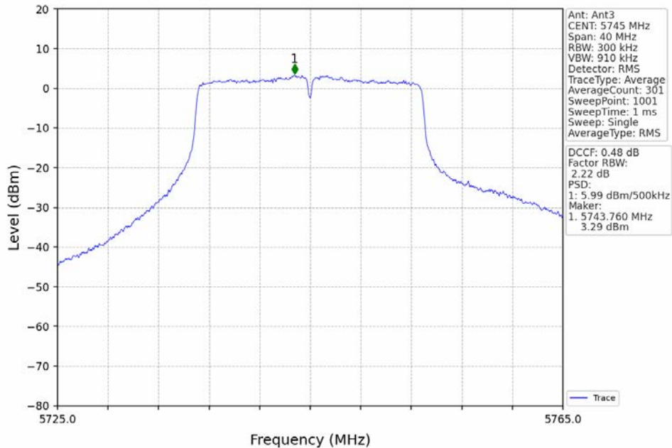
802.11ac(VHT20)_LCH_5745MHz_MIMO_NTNV
