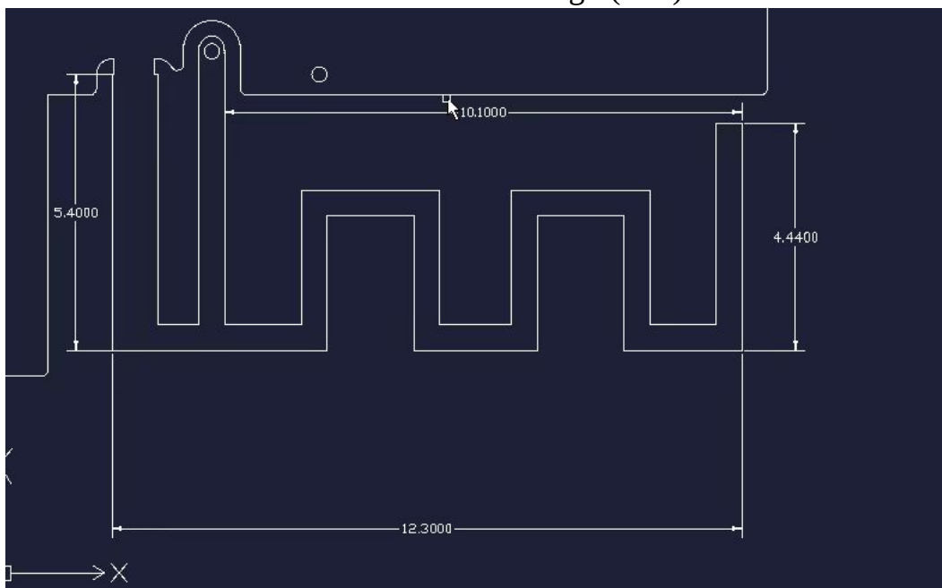
AntennaPhoto&Length(mm)
