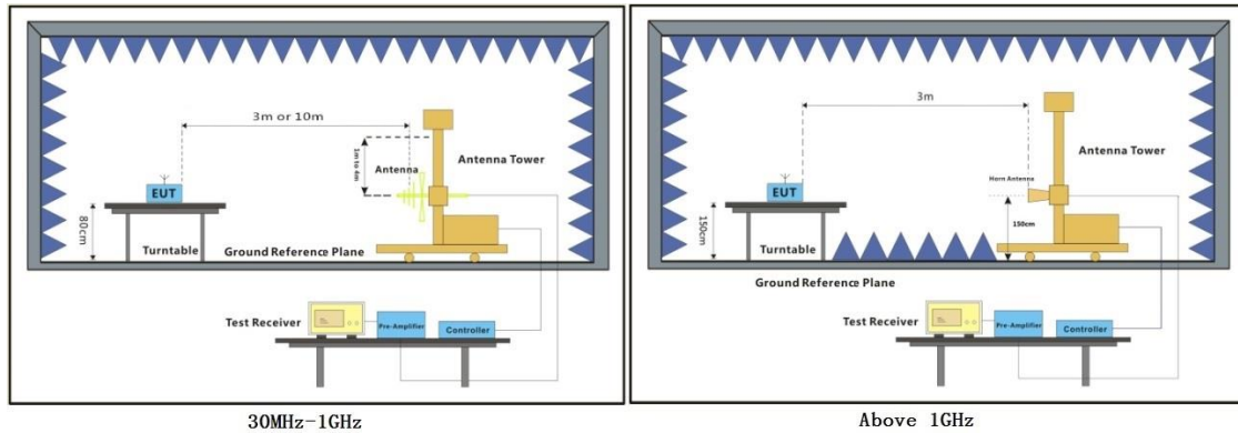
30MHz-1GHz
