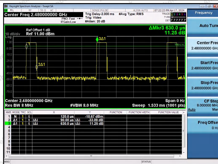
NTNV-BLE_1M-Ant1-2480
