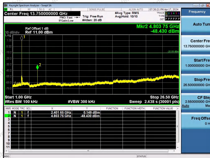
BLE_2M-Ant1-2402-1000~26500-PASS
