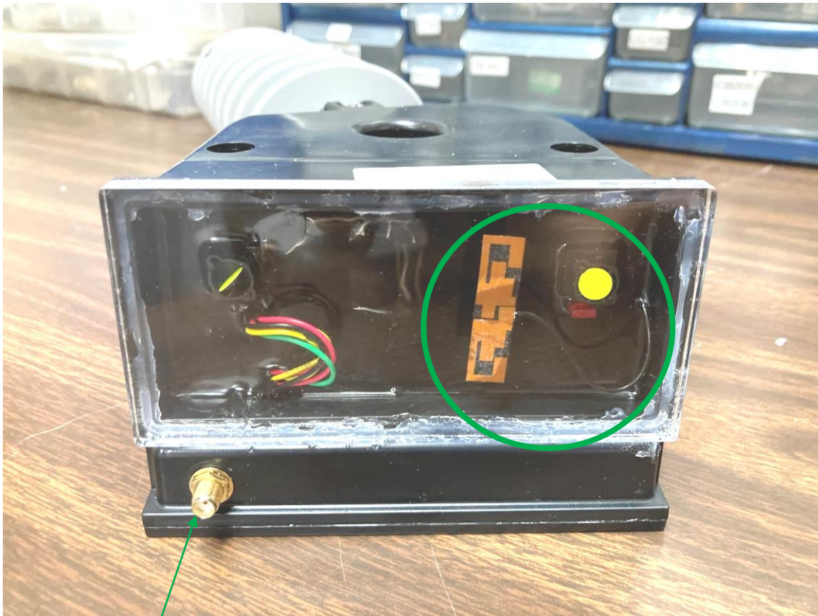
Figure 7. Antenna location in EUT
