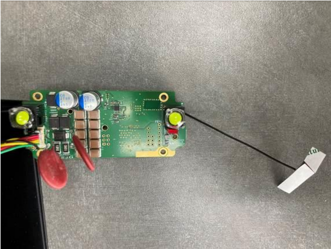
Figure 4. PCBA removed from case
