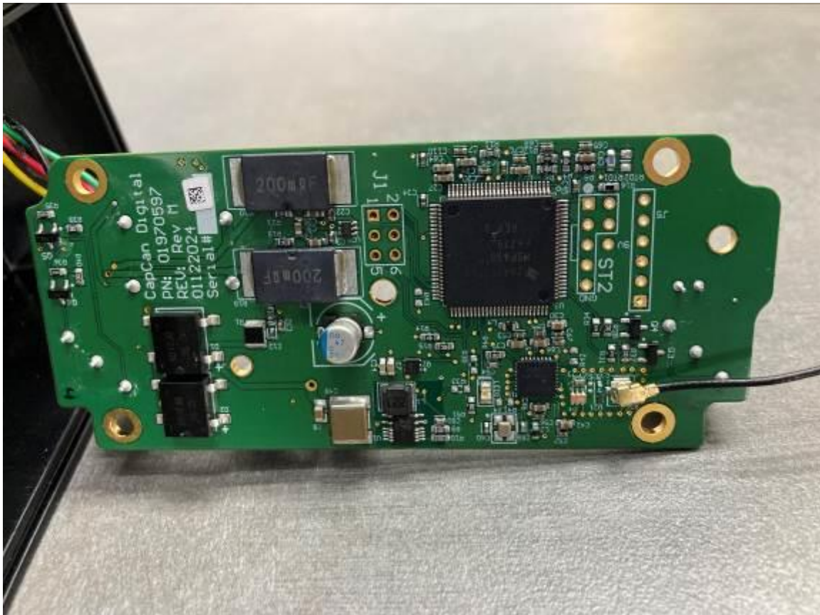
Figure 6. PCBA Bottom Side
