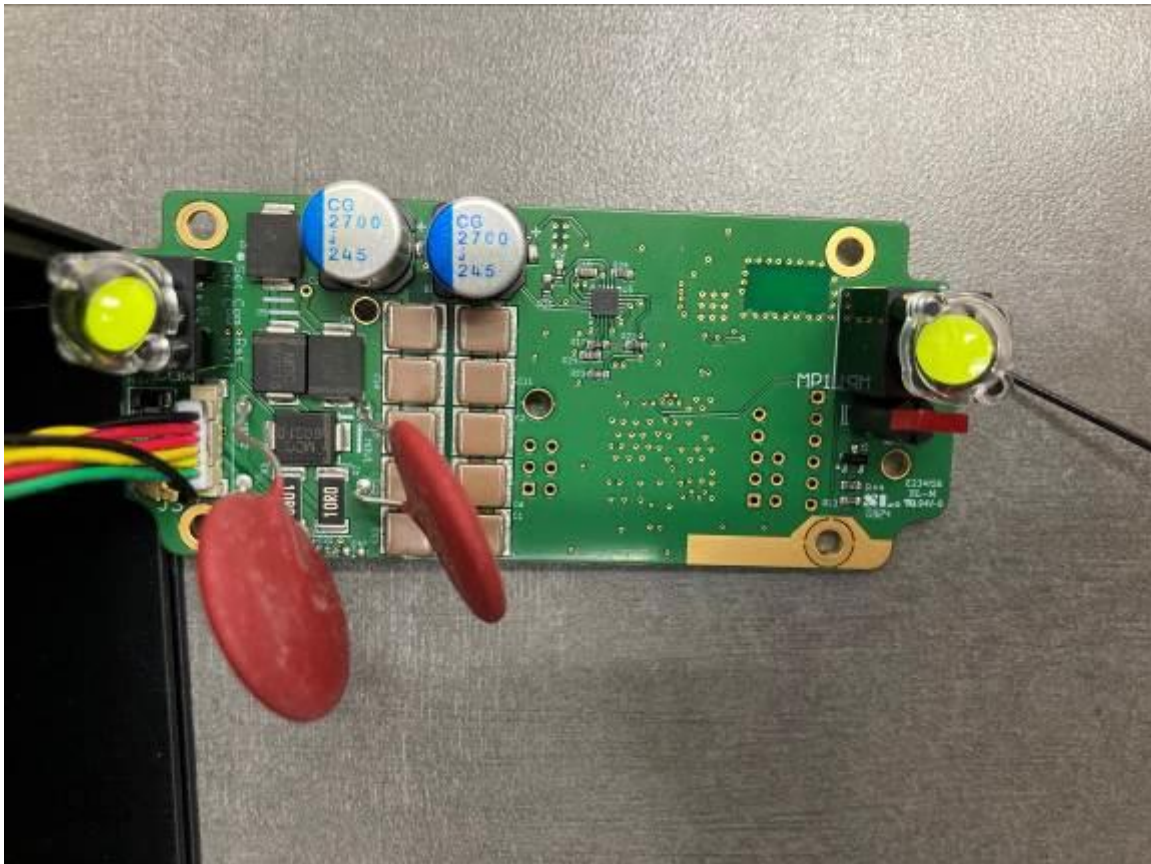
Figure 5. PCBA Top Side
