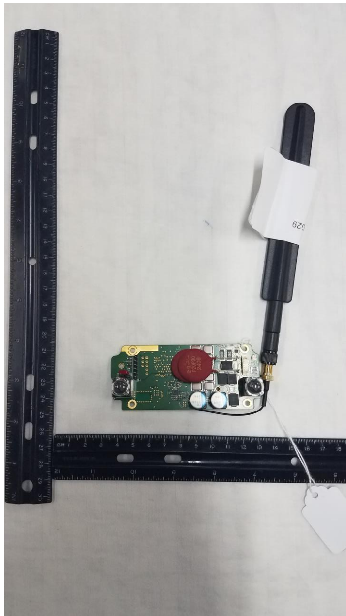
Figure 1. Front View
