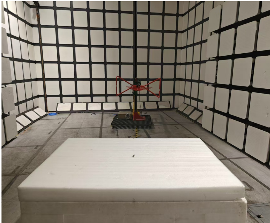
Radiated Emissions View (30 MHz-1 GHz)
