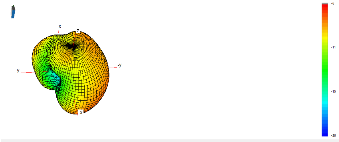
3D Antenna Pattern
