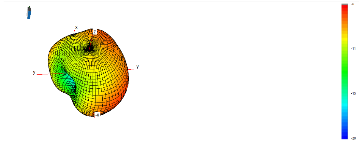
3D Antenna Pattern
