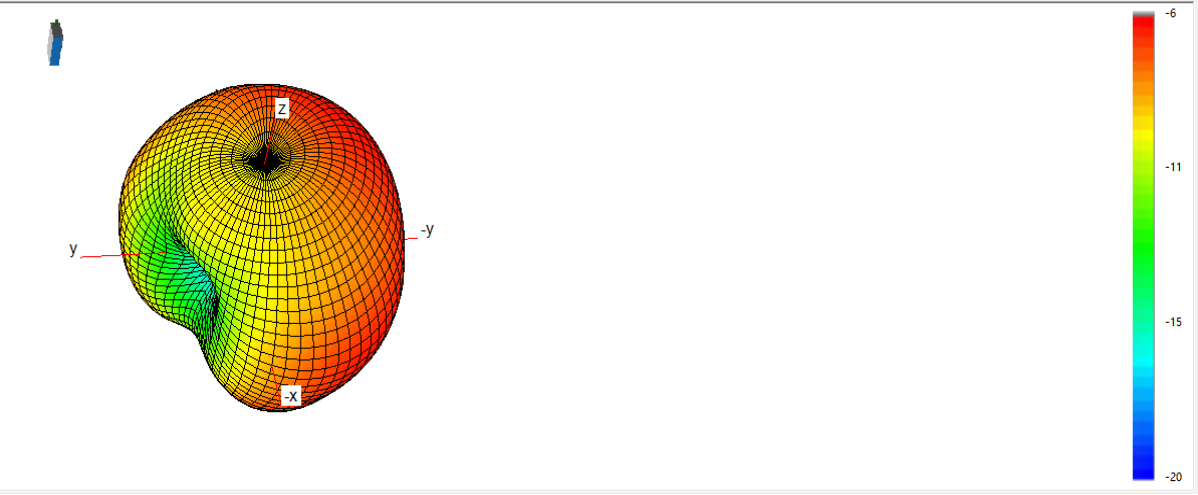
3D Antenna Pattern
