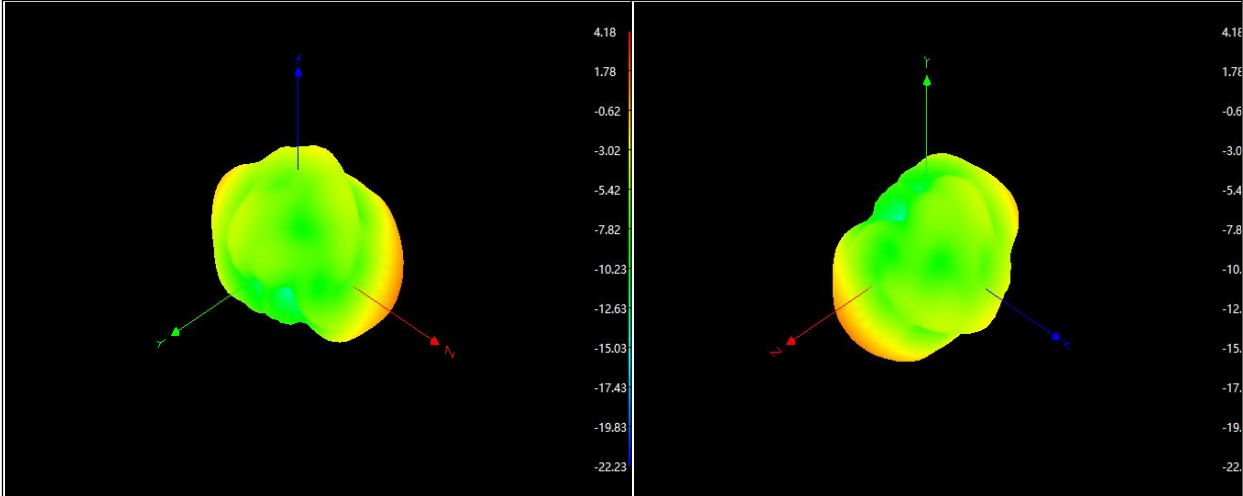
WiFi3: 2440Mhz
