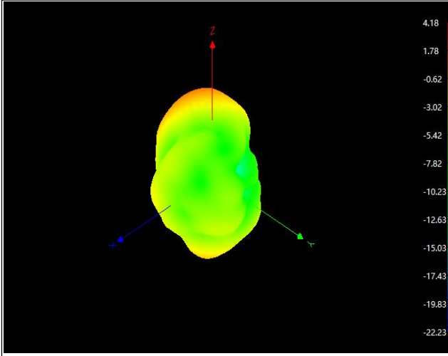
WiFi3: 2440Mhz
