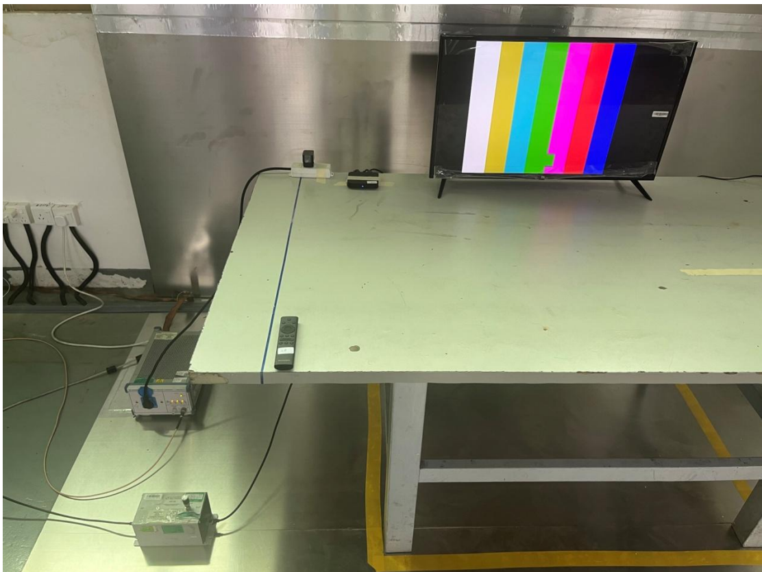
AC Conducted Measurement Photos
