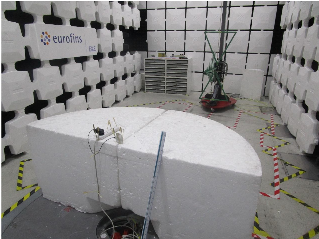
Radiated emissions tests 30MHz to 1GHz
