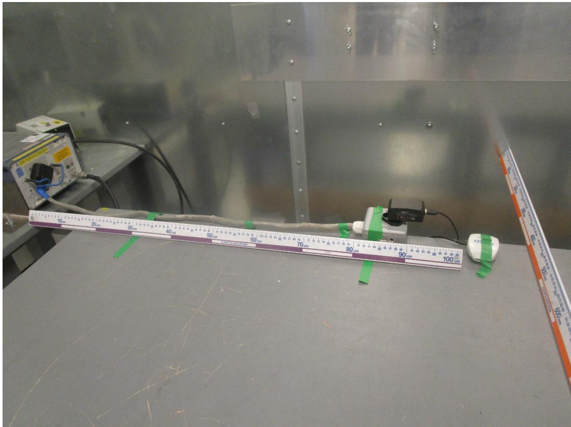
Mains conducted emissions tests 150kHz to 30MHz
