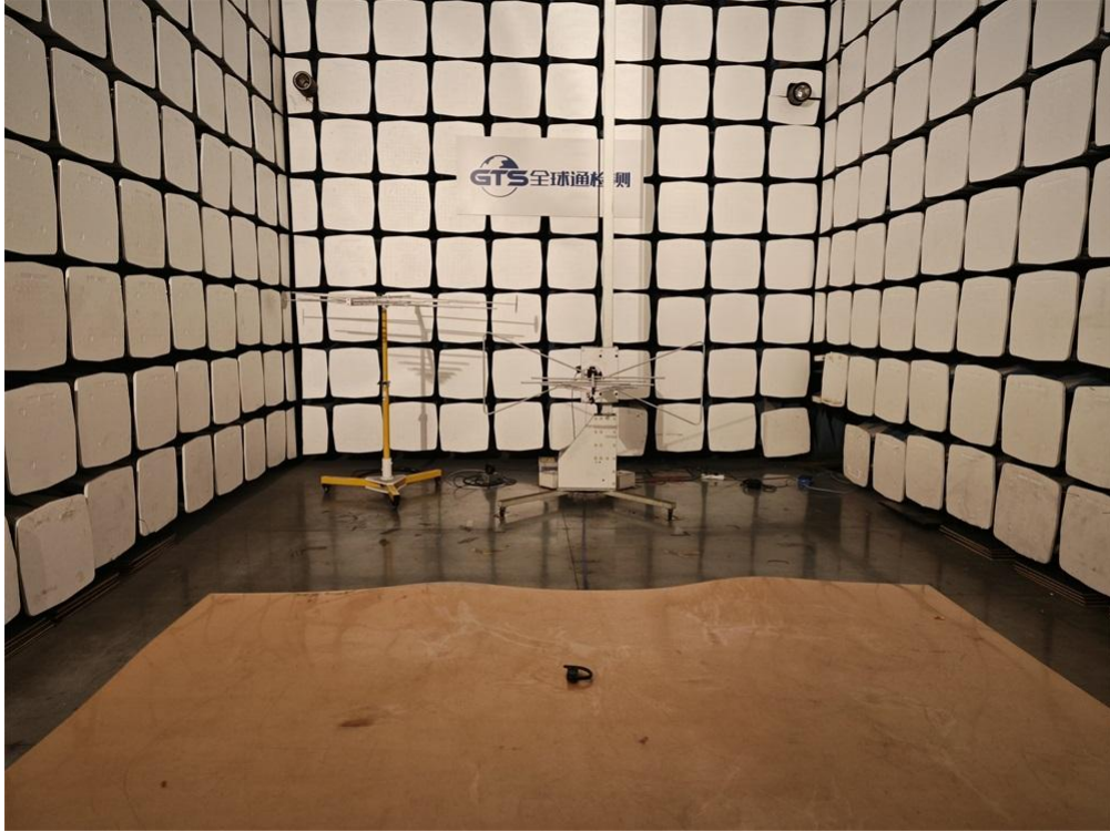
Photo of Radiated Emissions Measurement
