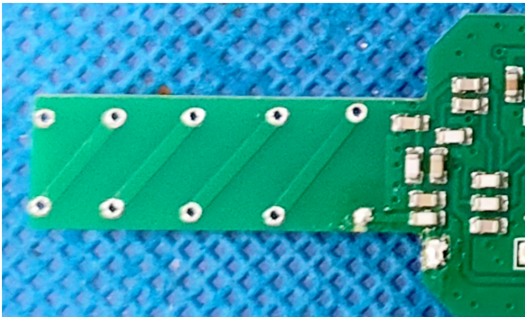
Antenna pictures
