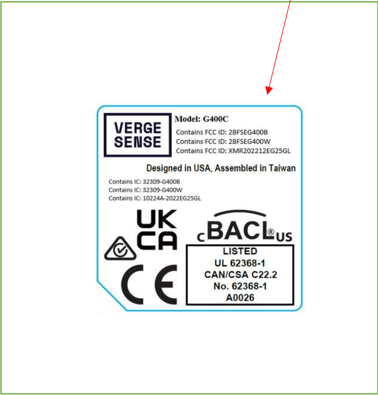
Host Device G400C Top View
