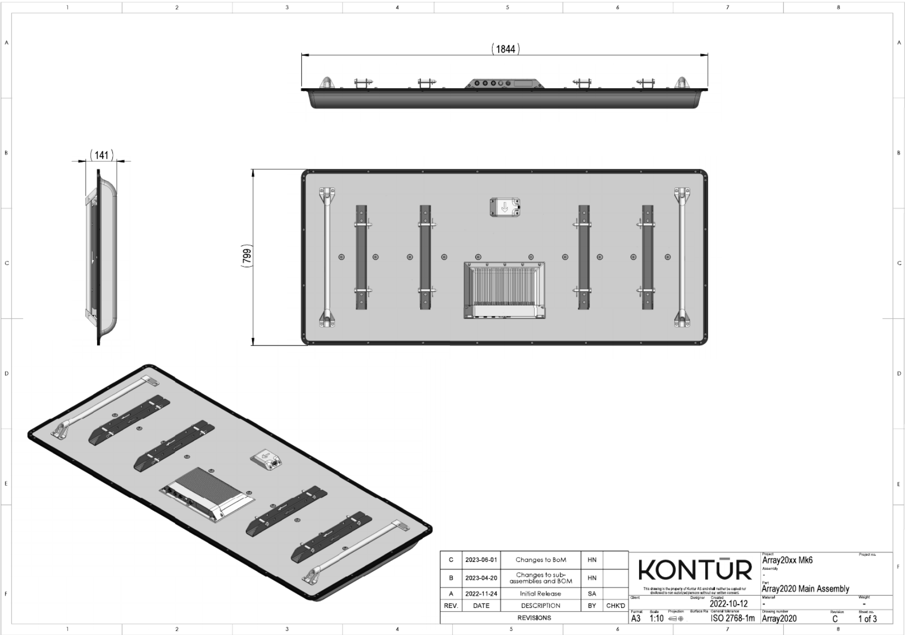
Figure 1: Antenna Specification – Ground 1820
