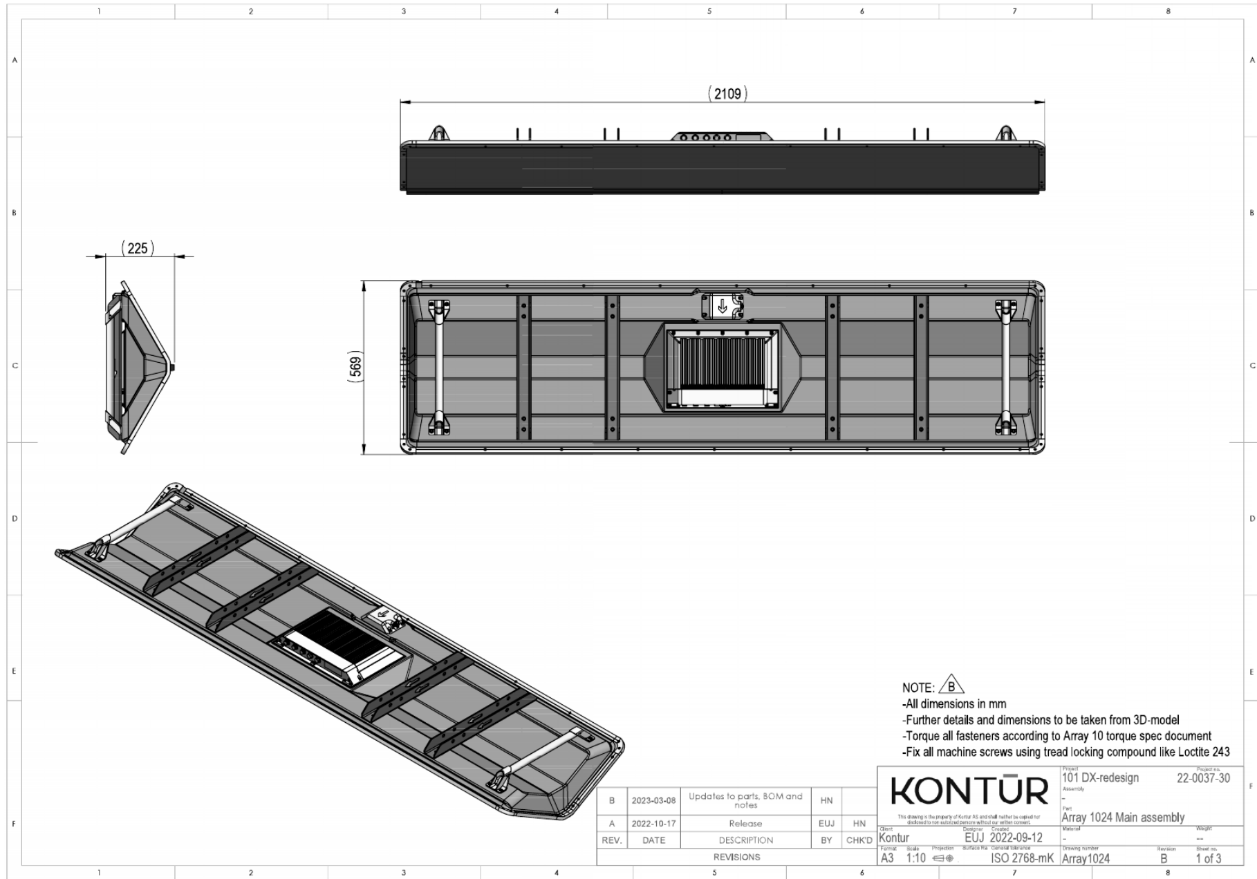
Figure 1: Antenna Specification – Air 2124
