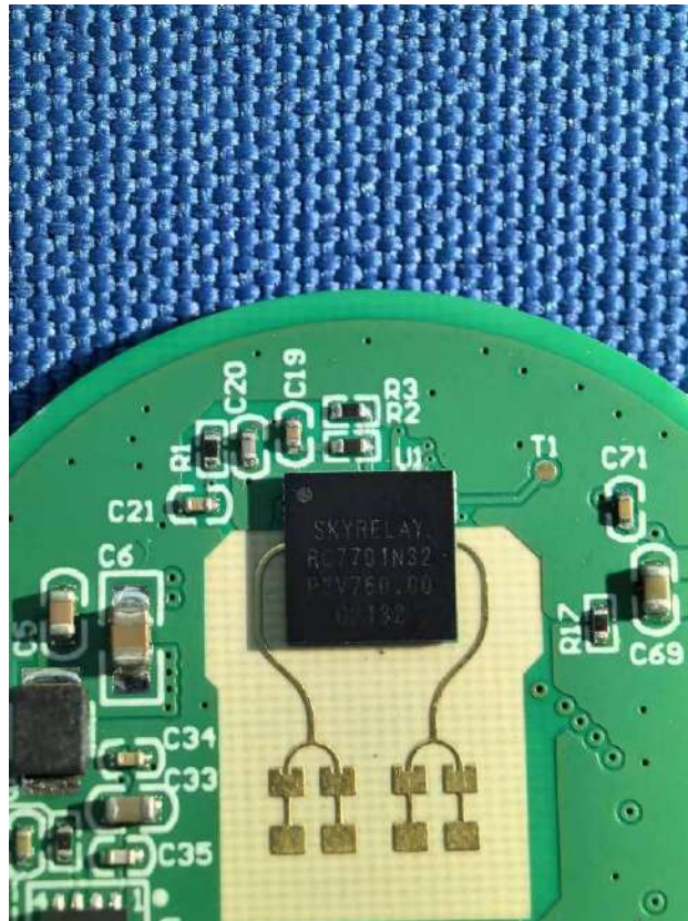
Radar Antenna
