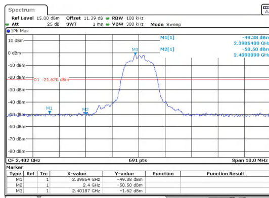
Out Of Band Emission \pi/4 QPSK_2-DH5_Channel 0
