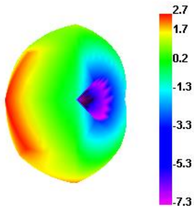
Bluetooth 78 TRP
