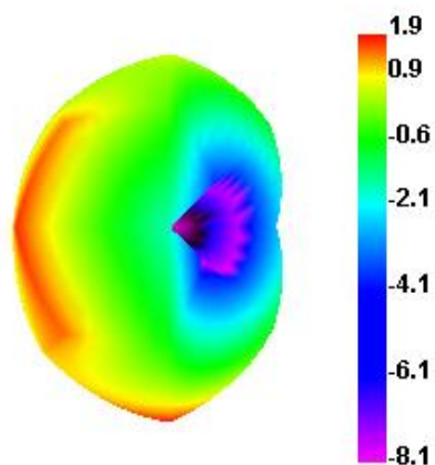
Bluetooth 39 TRP
