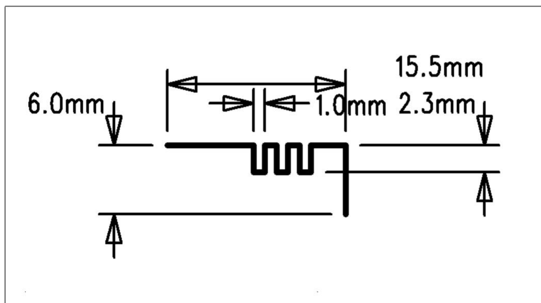
AntennaPhoto&Length(mm)
