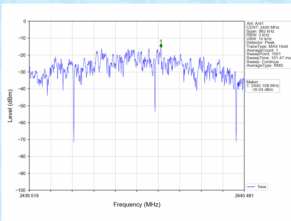
1M_MCH_2440MHz_Ant1_NTNV
