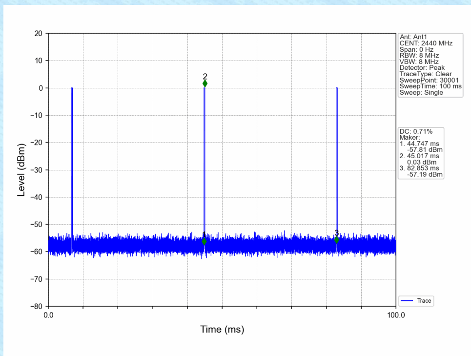
1M_MCH_2440MHz_Ant1_NTNV
