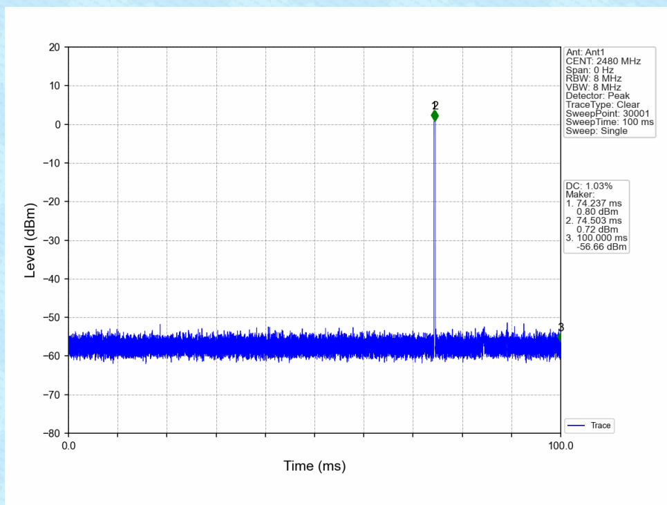
1M_HCH_2480MHz_Ant1_NTNV
