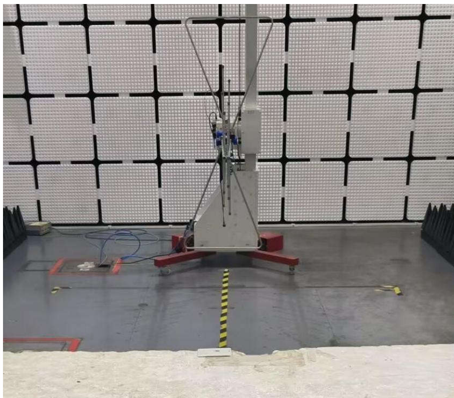
Radiated spurious emission Test Setup-2(Below 1GHz)Close up photo
