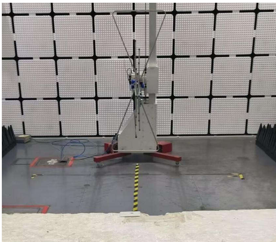
Radiated spurious emission Test Setup-2(Below 1GHz) close up
