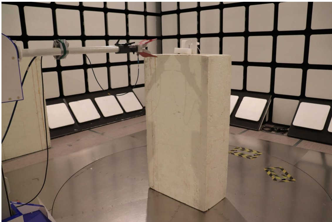
Photograph 5. Radiated emissions 1000 – 1610 MHz and 10.6 – 18 GHz
