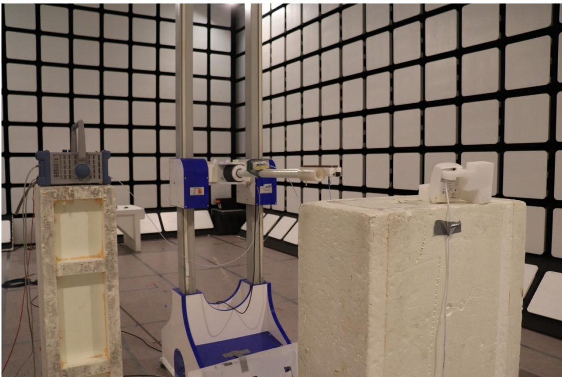
Photograph 8. Radiated emissions 26.5 – 40 GHz
