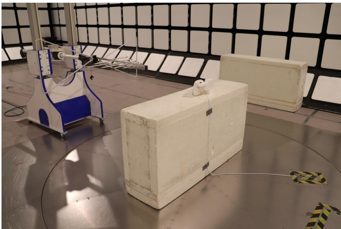
Photograph 4. Radiated emissions 960 – 1000 MHz
