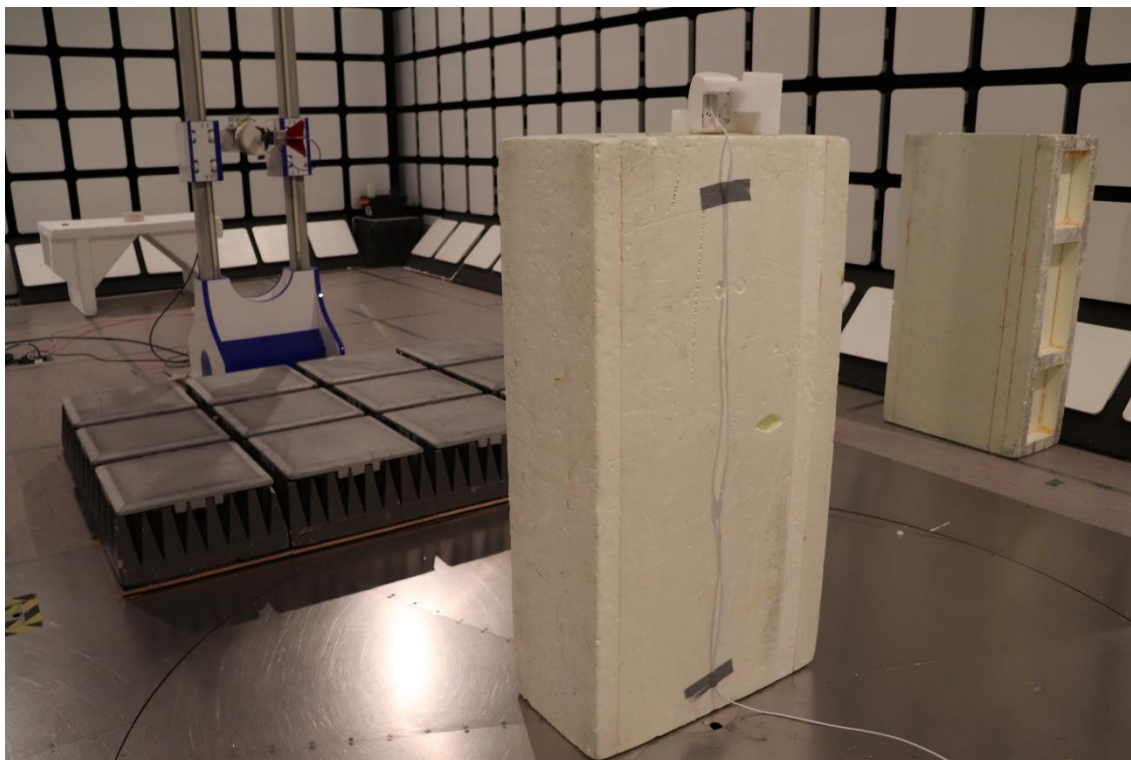
Photograph 6. Radiated emissions 1164 – 1240 MHz, 1559 – 1610 MHz, 1610 – 3500 MHz, and 4.5 – 10.6 GHz
