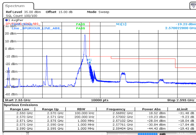
20MHz_High_QPSK_1@99 -19.23dBm
