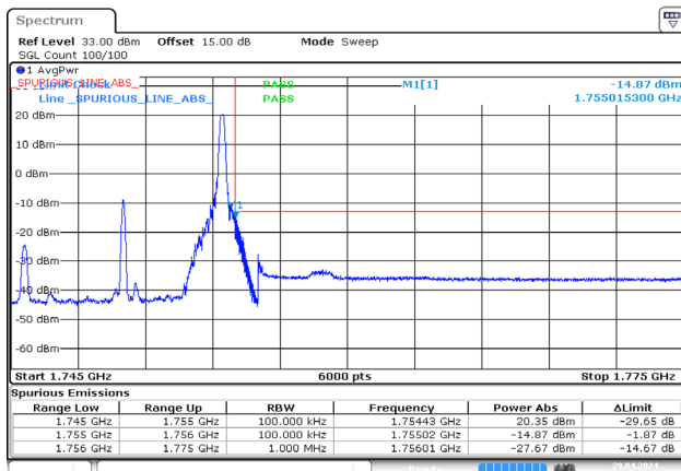
10MHz_High_QPSK_1@49 -14.87dBm
