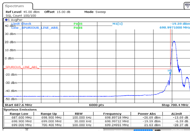
1.4MHz_Low_QPSK_1@0 -19.59dBm
