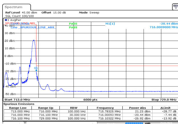
3MHz_High_QPSK_1@14 -20.44dBm
