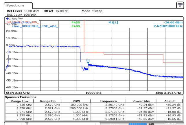
20MHz_High_QPSK_100@0 -26.60dBm
