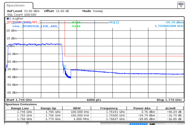
10MHz_High_QPSK_50@0 -29.79dBm
