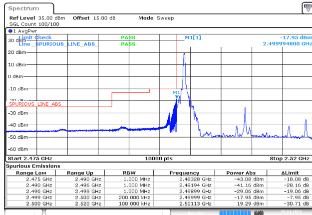
20MHz_Low_QPSK_1@0 -17.95dBm
