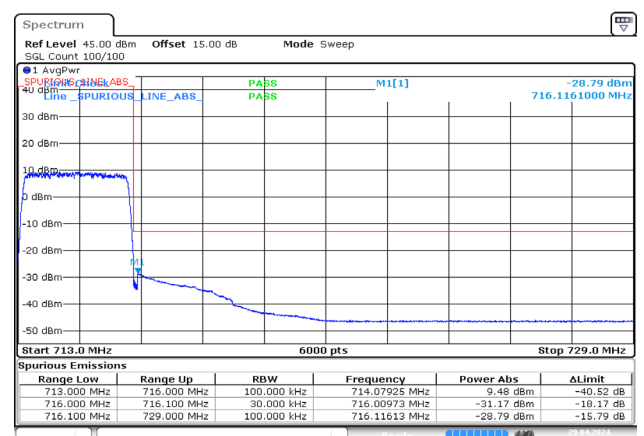
3MHz_High_QPSK_15@0 -28.79dBm
