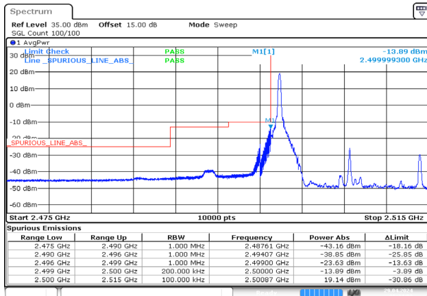
15MHz_Low_QPSK_1@0 -13.89dBm
