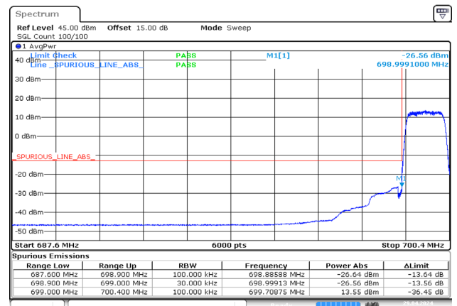
1.4MHz_Low_QPSK_6@0 -26.56dBm
