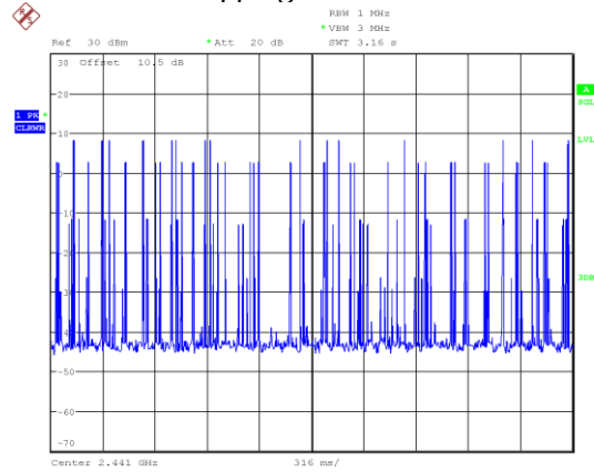
Hopping Numbers-2DH3
