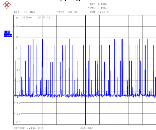
Hopping Numbers-2DH5
