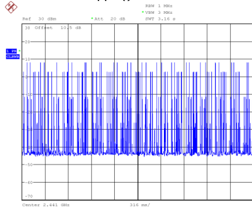
Hopping Numbers-2DH1
