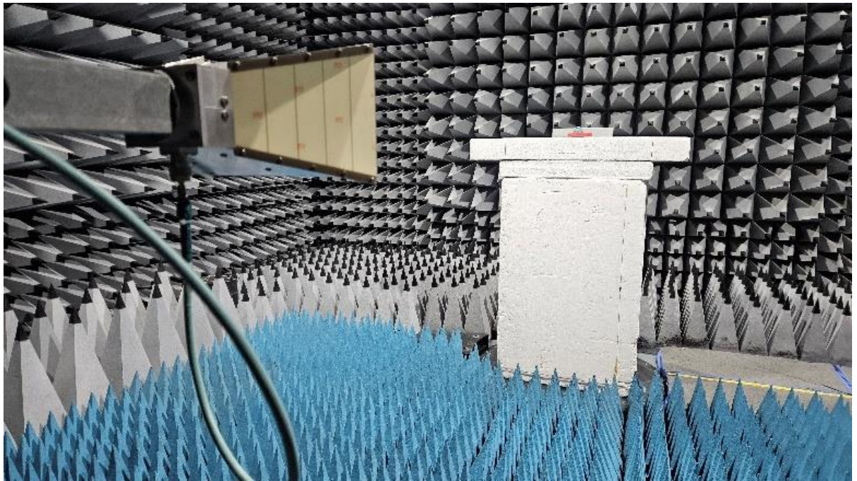
Radiated Emissions 1GHz -18GHz
