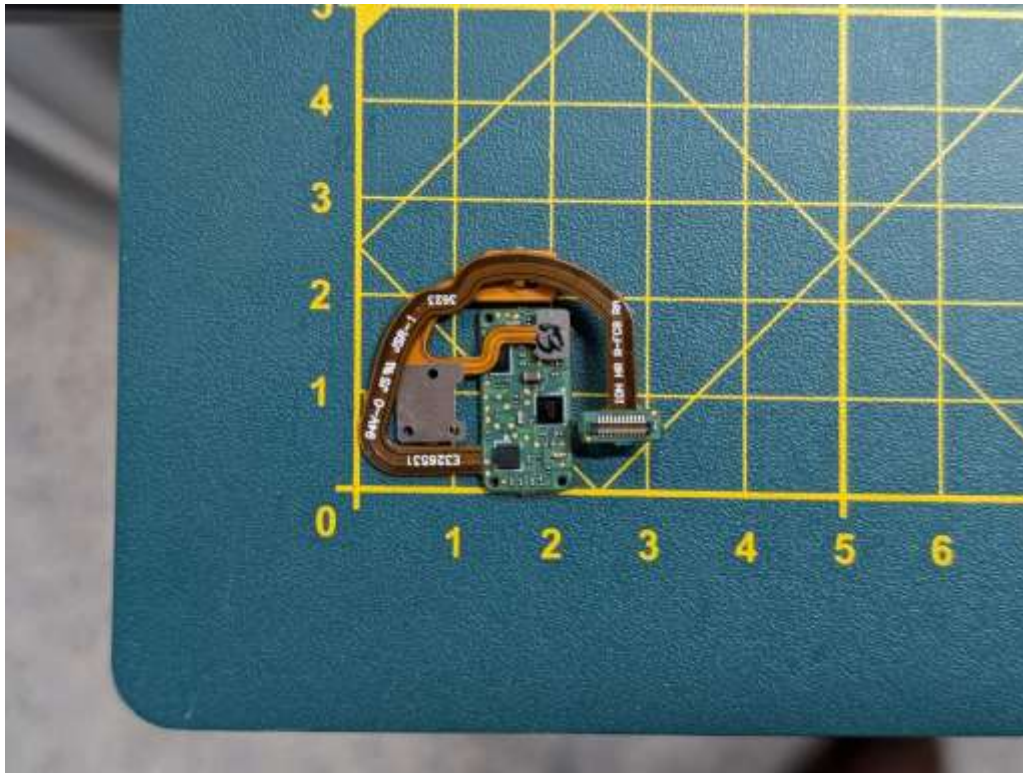
HR board bottom view
