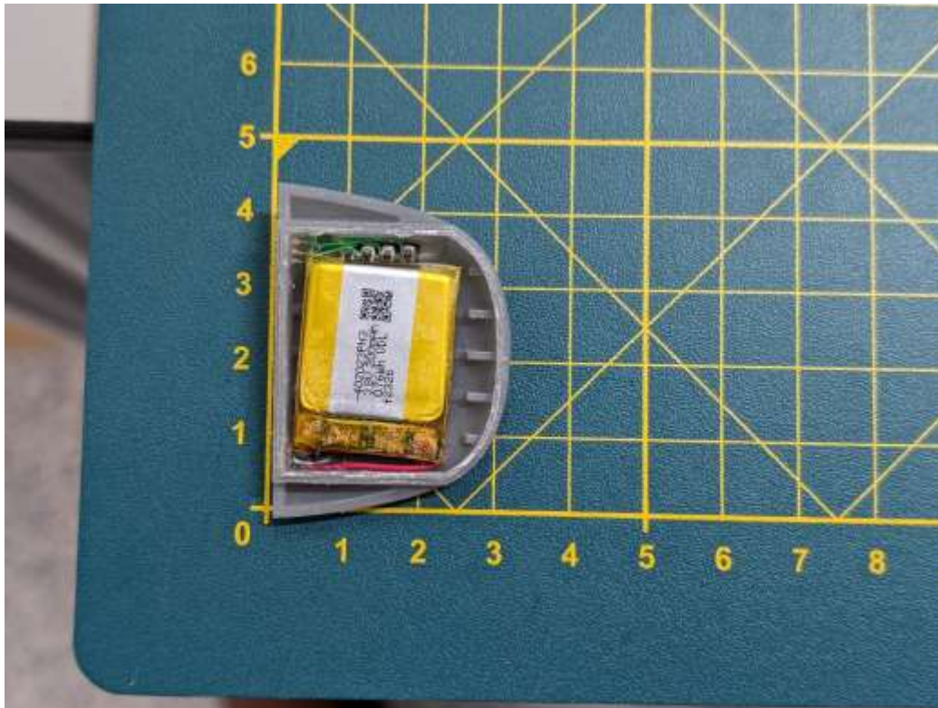
Battery housing inside test pins visible
