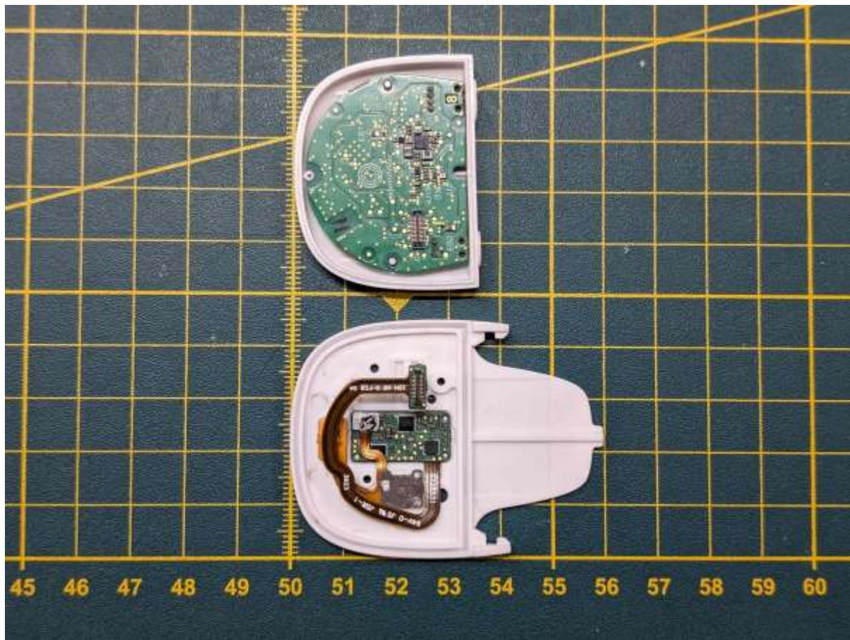
IDH housing internal
