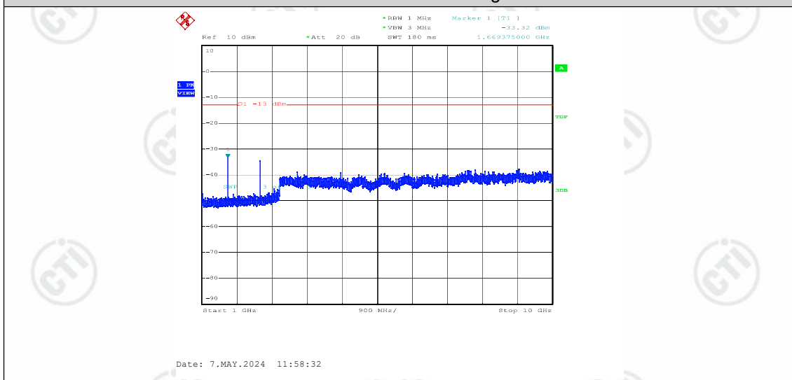
Band26-15MHz-16QAM-26965-1RB#0-Range2:1000~10000MHz
