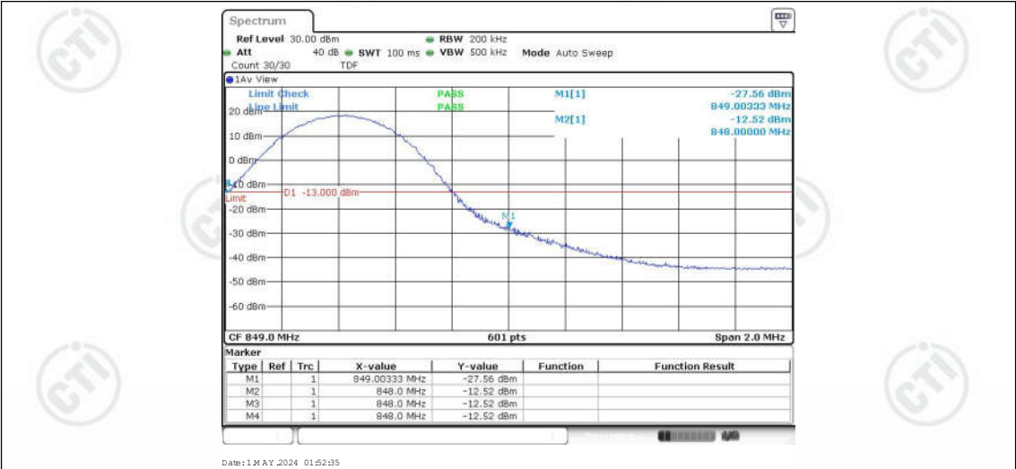
Band26-10MHz-16QAM-26990-50RB#0
