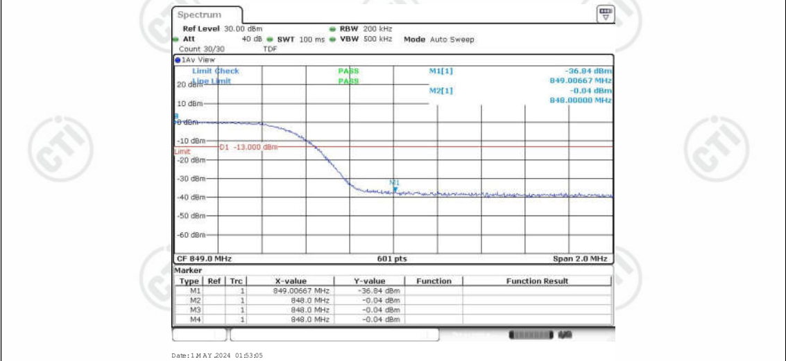
Band26-15MHz-QPSK-26965-1RB#0
