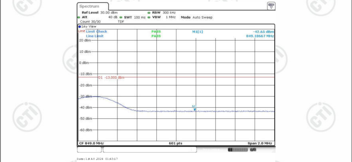
Band26-15MHz-QPSK-26965-1RB#0
