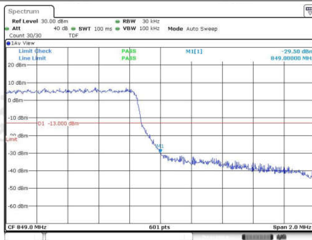
Band26-1.4MHz-16QAM-27033-1RB#0
