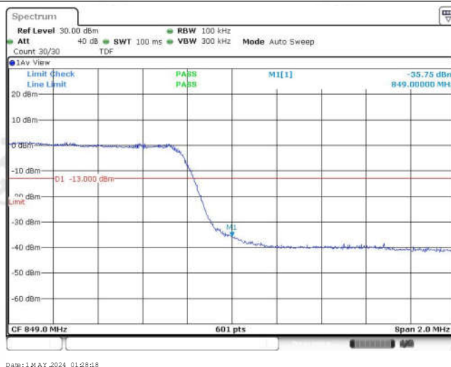
Band26-10MHz-QPSK-26990-1RB#0
