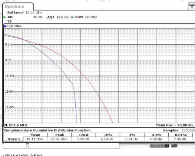
Band26-10MHz-16QAM-26865-50RB#0
