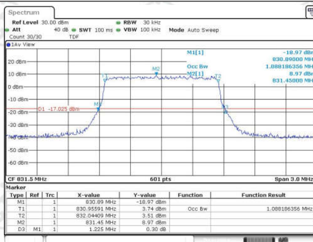
Band26-1.4MHz-QPSK-26865-6RB#0-1.088
