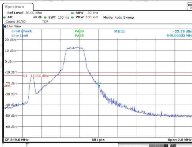
Band26-1.4MHz-16QAM-27033-1RB#5
