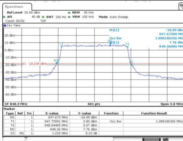
Band26-1.4MHz-QPSK-27033-6RB#0-1.088
