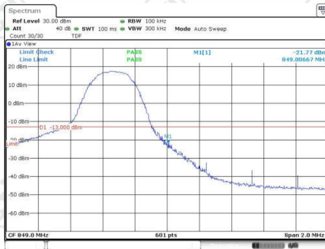
Band26-5MHz-QPSK-27015-1RB#24
