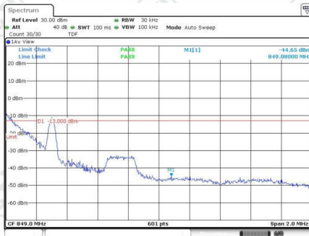
Band26-1.4MHz-16QAM-27033-1RB#0
