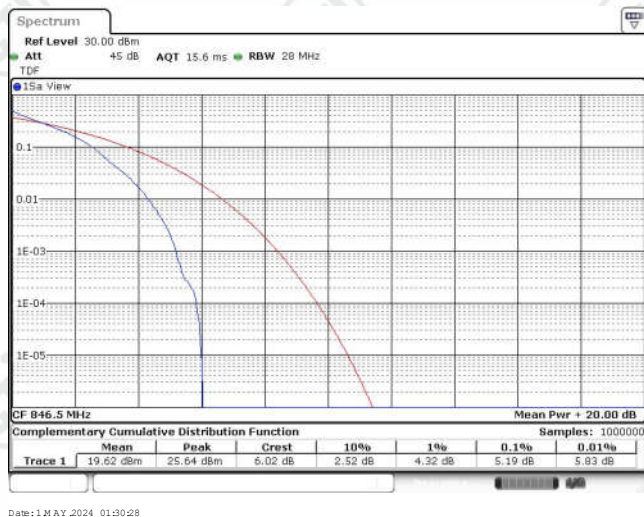
Band26-5MHz-QPSK-27015-25RB#0
