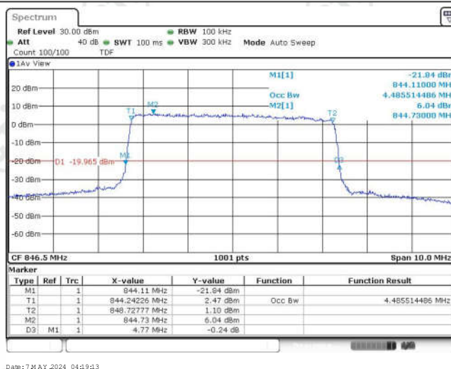
Band26-5MHz-QPSK-27015-25RB#0-4.486
